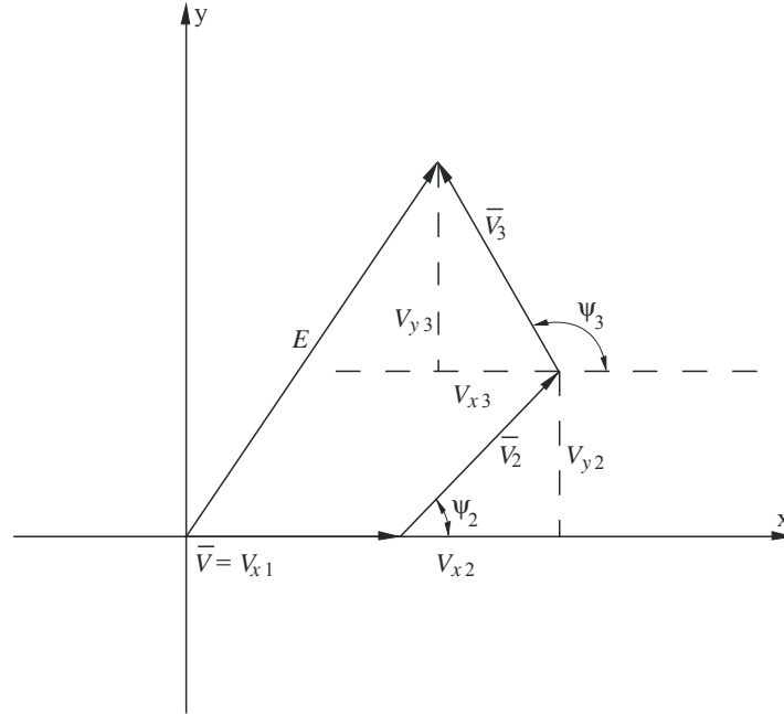
FIGURE 23 x-y plane vectorial addition for n = 3
