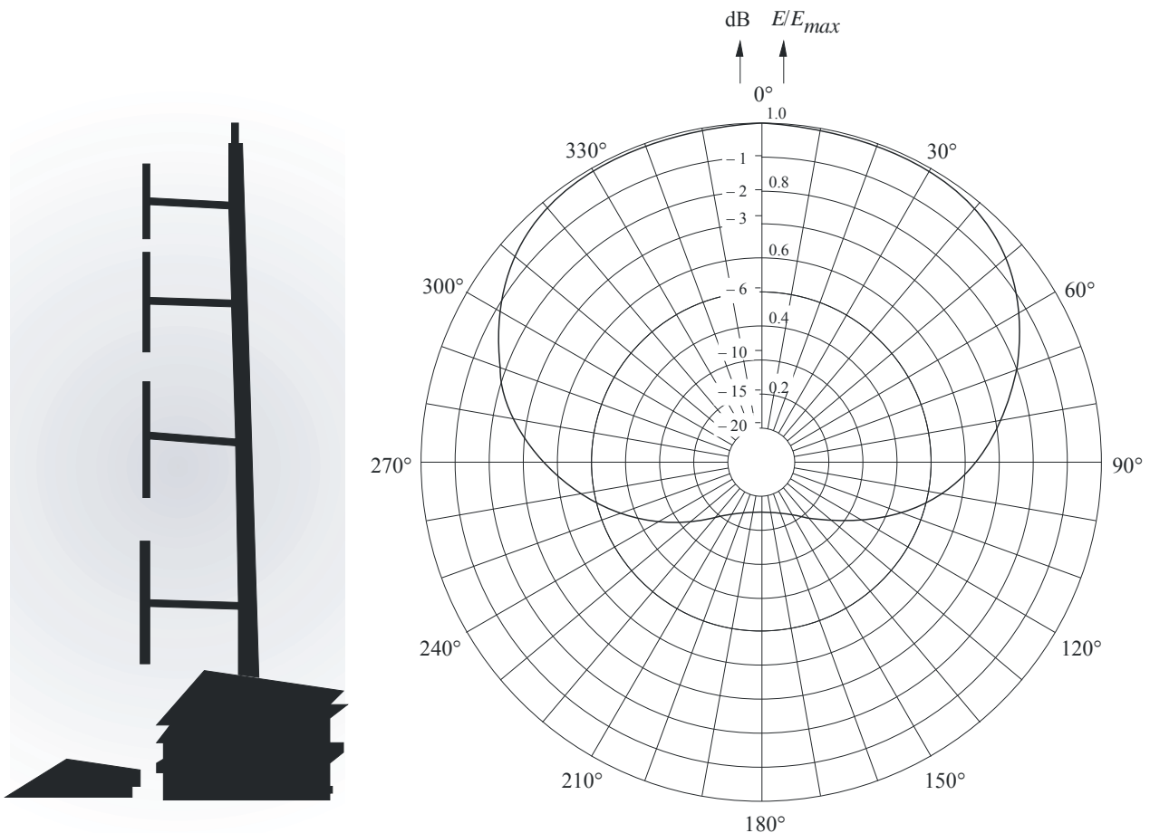
FIGURE 24 Vertically polarized Band II dipole antenna
