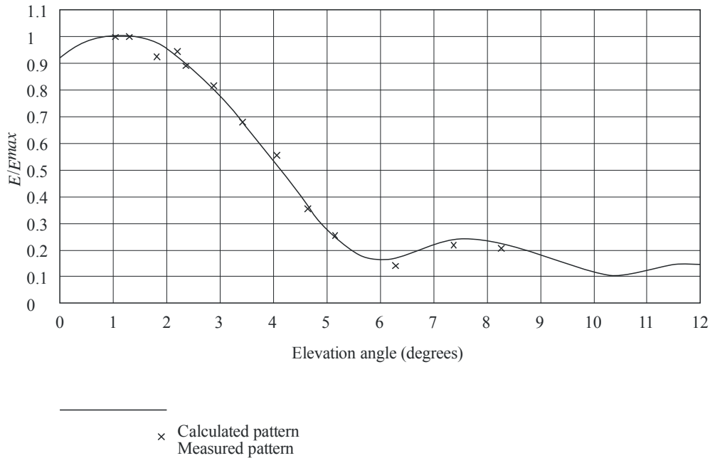
FIGURE 41 Calculated and measured vertical patterns
