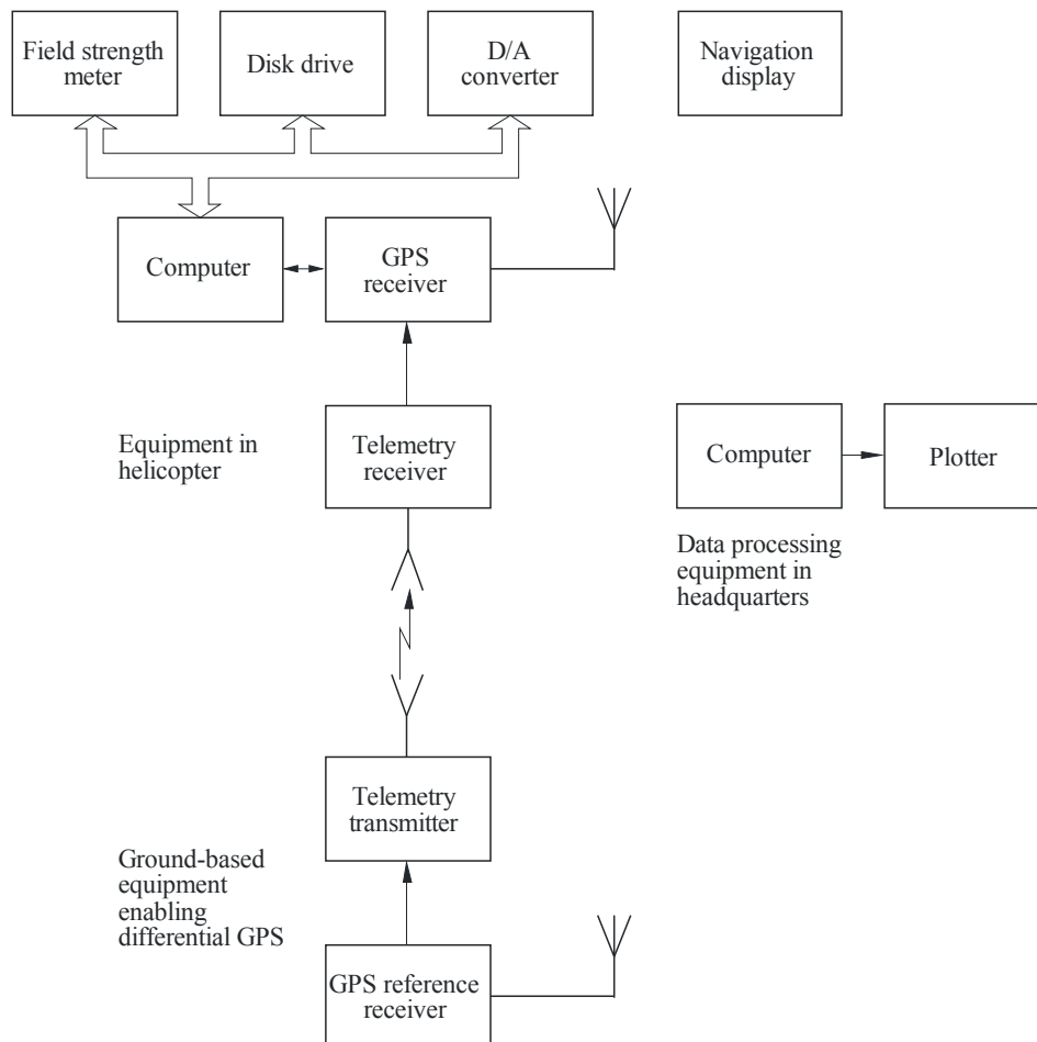
Block diagram of the measuring equipment
