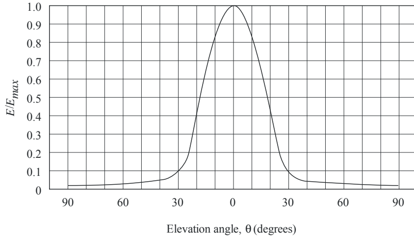
Vertical radiation pattern of the array of Fig. 19 when a binomial amplitude distribution is applied
