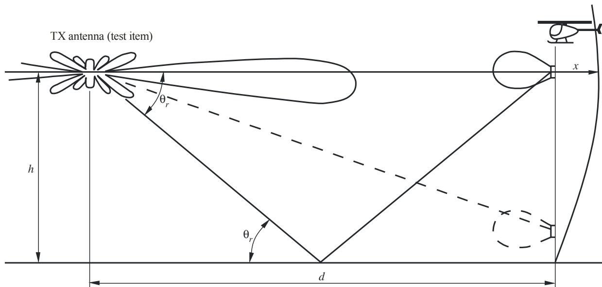
FIGURE 44 Representation of flight path
