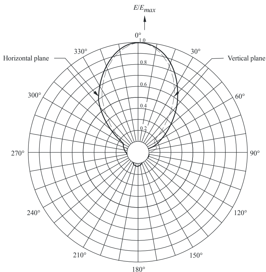
FIGURE 17 Vertical and horizontal radiation patterns of the dipole panel of Fig. 16
