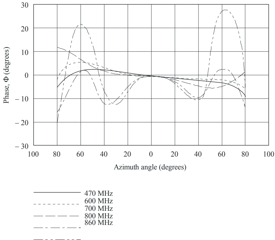
Phase patterns of a wideband UHF panel antenna at various operating frequencies
