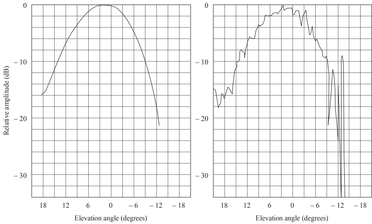
Calculated and measured vertical patterns
