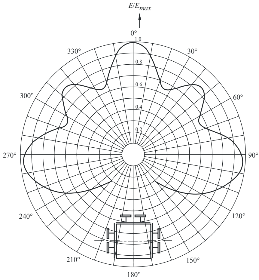
FIGURE 29 Directional azimuth pattern of a 3-panel antenna system in Band III
