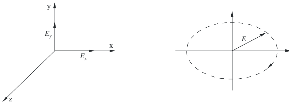
FIGURE 4 Elliptical polarization
