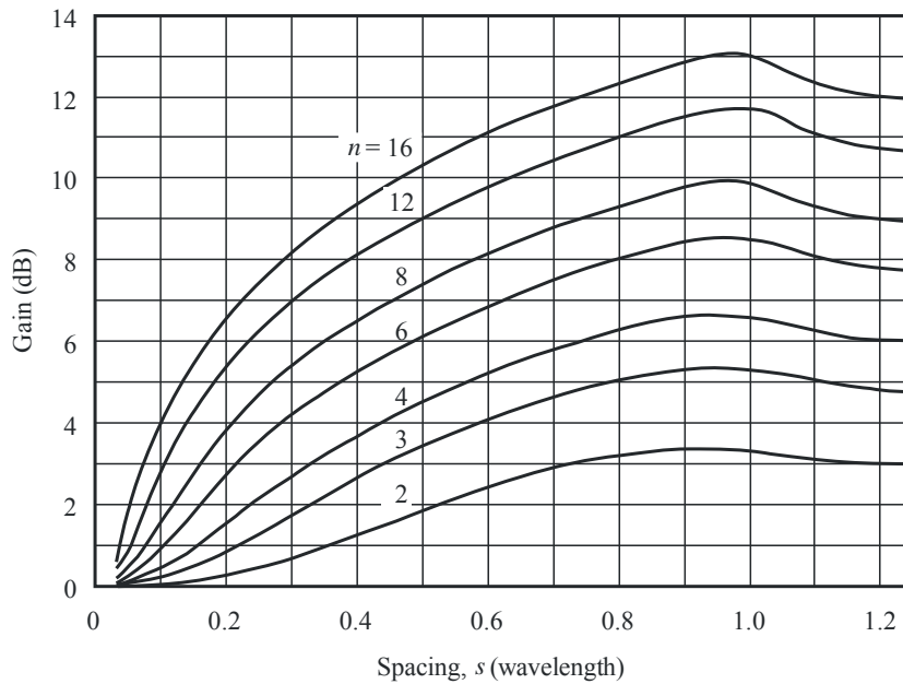
FIGURE 11 Gain of a vertical collinear array as a function of the number n of elements and their spacing s . The gain is referred to that of a single element
