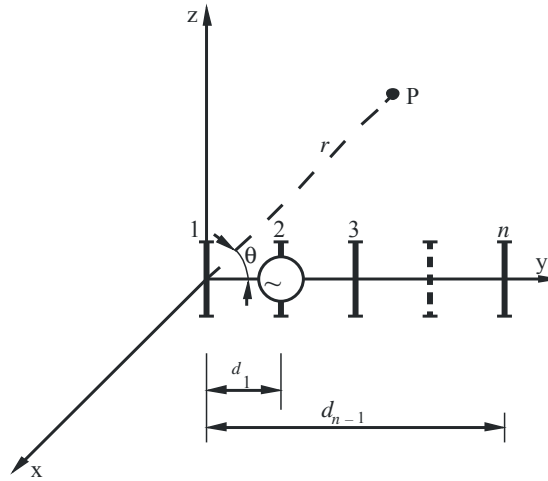
FIGURE 12 Yagi antenna
