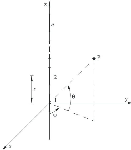
FIGURE 10 Omnidirectional collinear array
