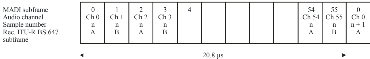
FIGURE 2 48 kHz with 56 channels working
