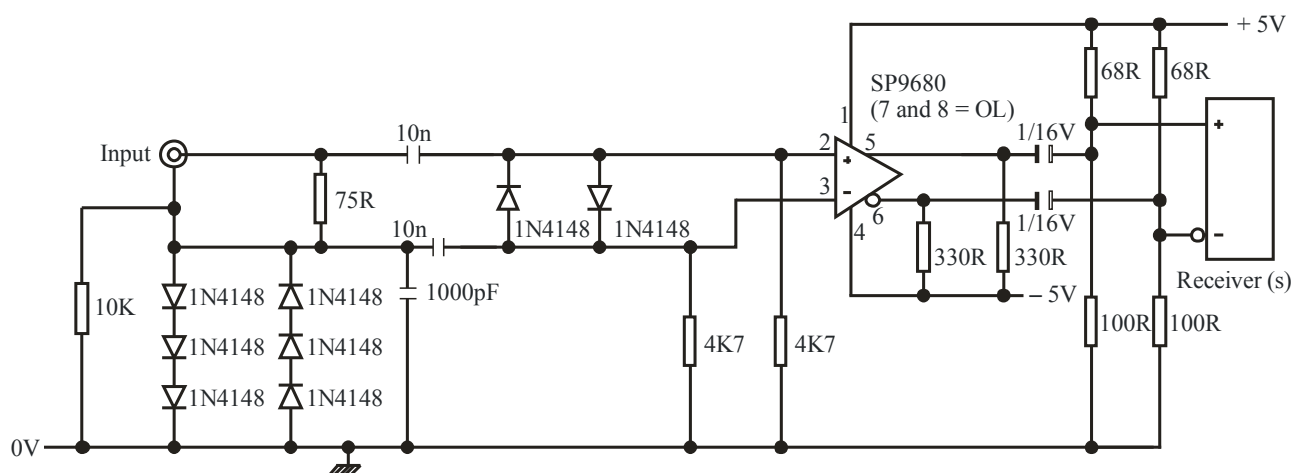
FIGURE 8 MADI buffer circuits (informative)
