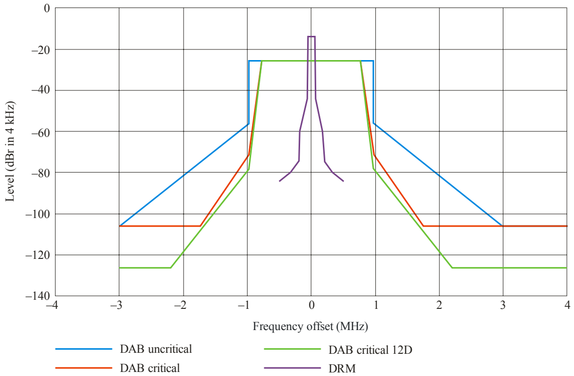
Out-of-band spectrum masks for DAB and DRM in VHF Band III
