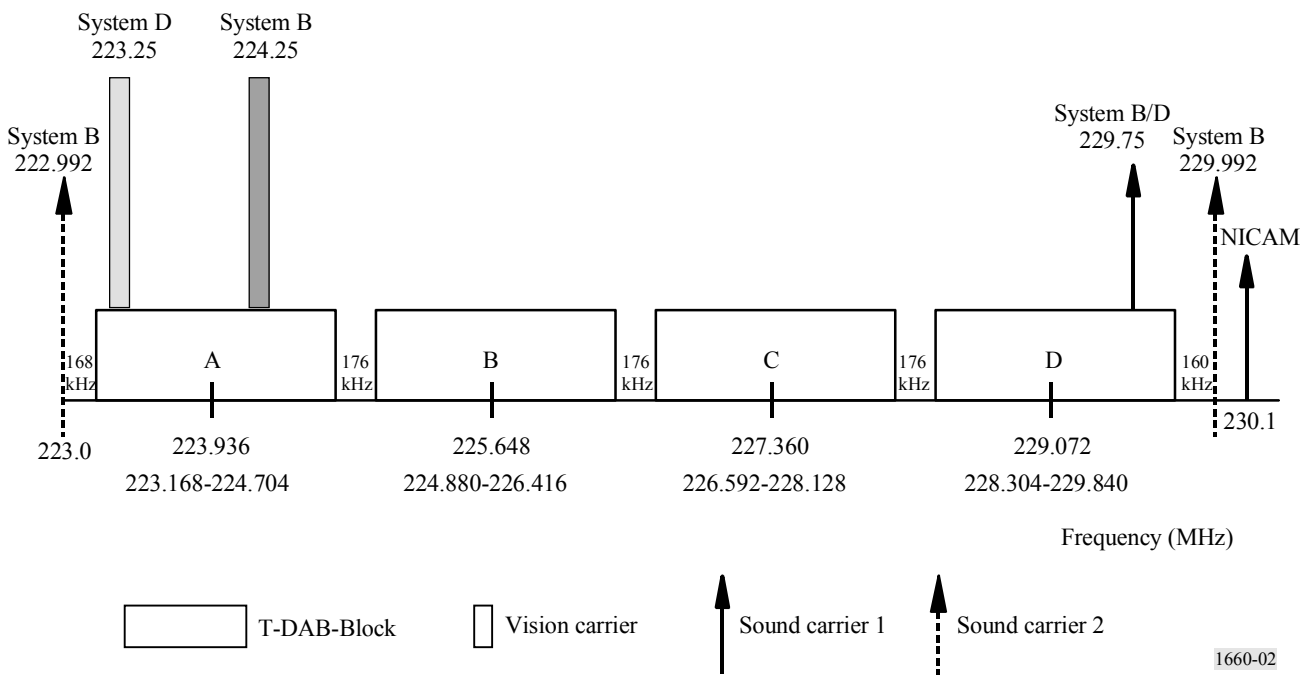
FIGURE 2 Position of T-DAB blocks in channel 12
