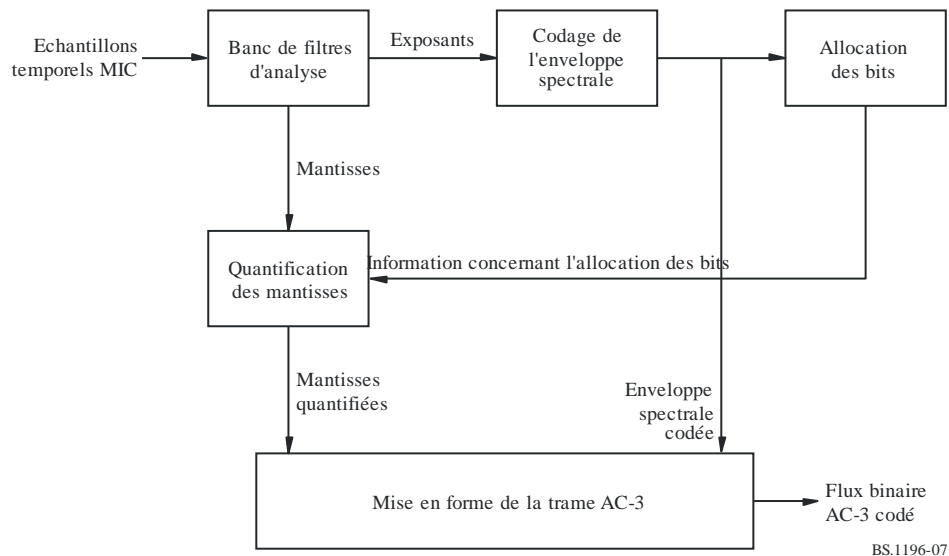
FIGURE 7 Codeur AC-3
