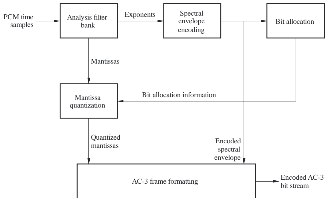
FIGURE 7 The AC- encoder
