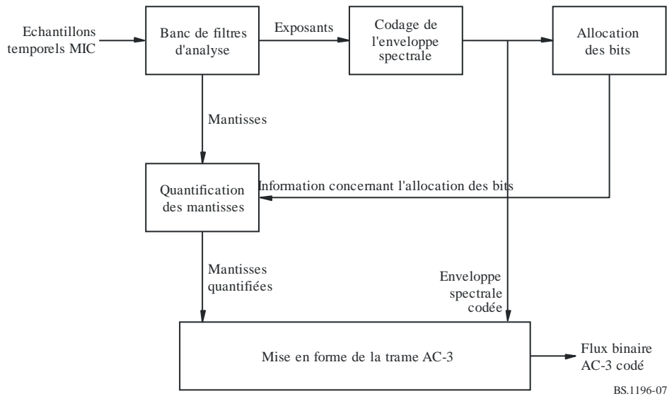
FIGURE 7 Codeur AC-3
