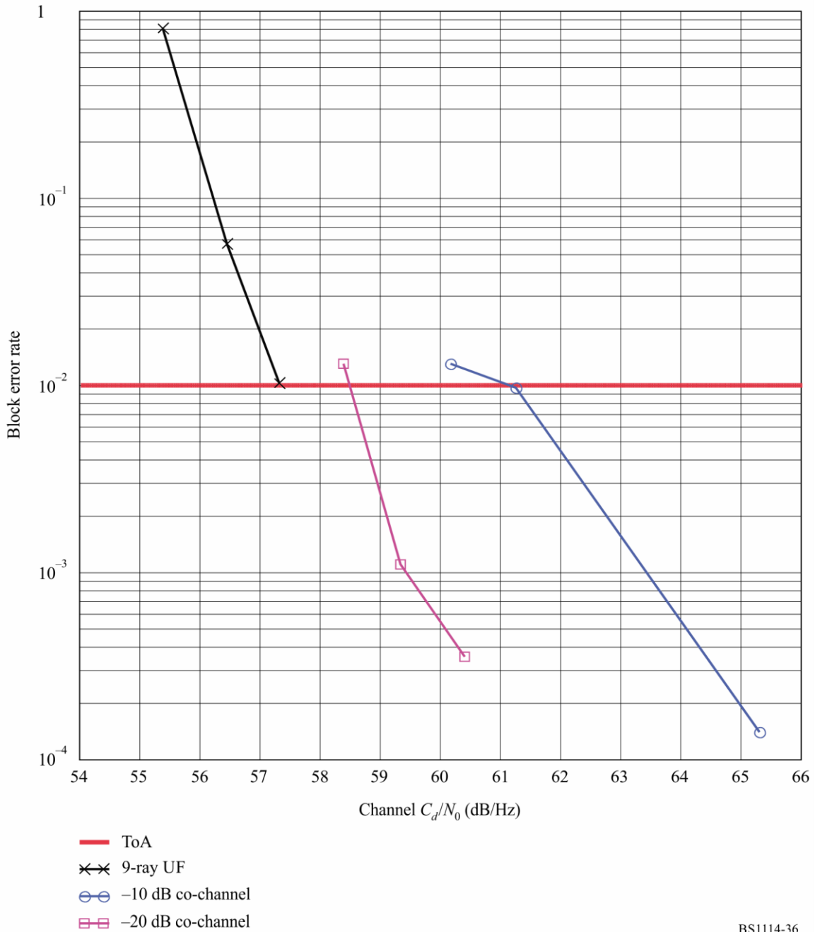
FIGURE 36 Block error rate results of the hybrid system with an independently faded 10-channel interferer
