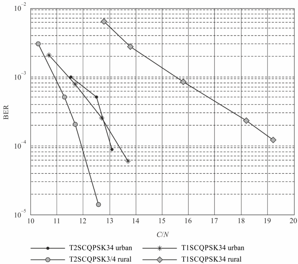
FIGURE 55 BER vs. C/N in multipath channel
