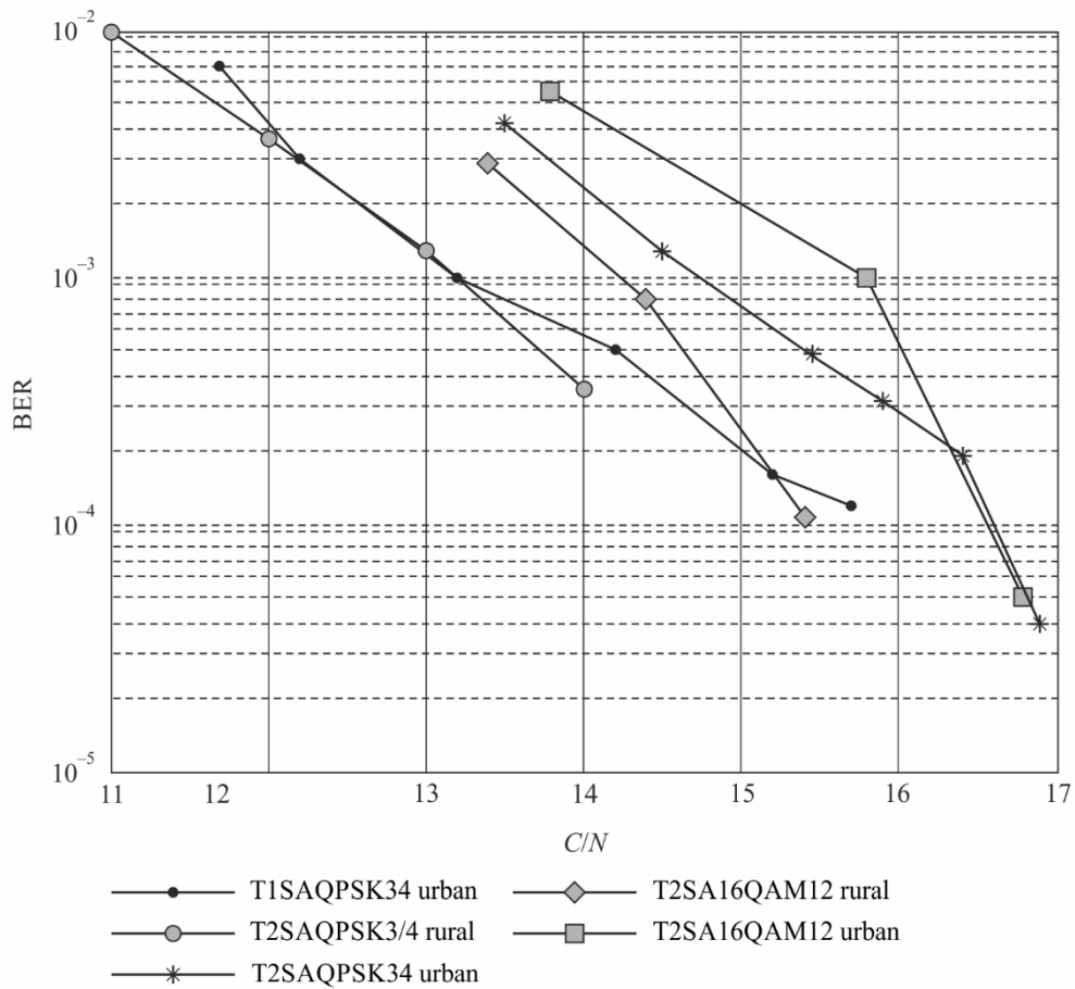
BER vs. C/N in multipath channel
