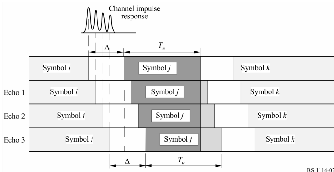
FIGURE 2 Constructive contribution of echoes
