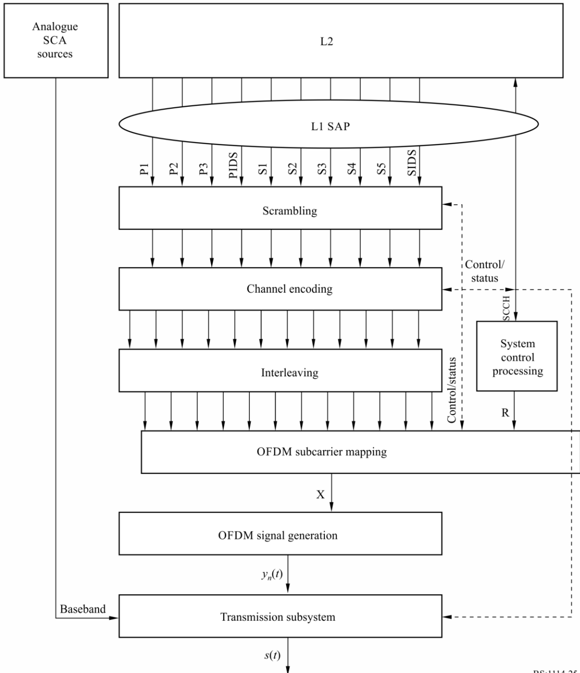
FIGURE 25 FM air interface L1 functional block diagram
