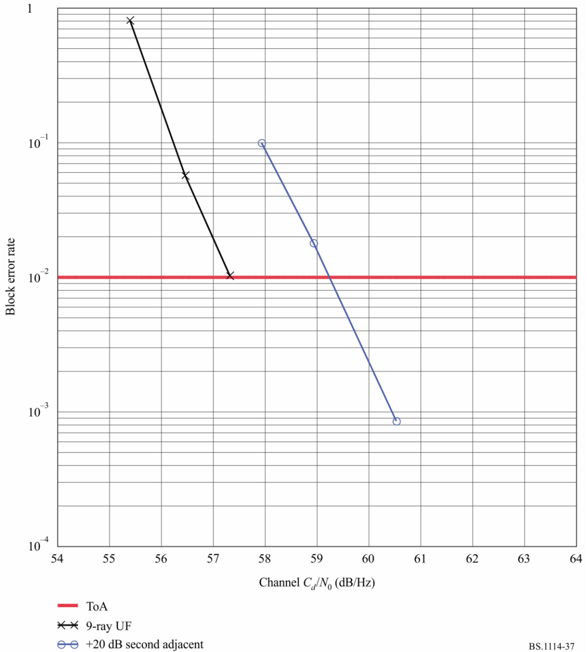
FIGURE 37 Block error rate results of the hybrid system with an independently faded second-adjacent interferer
