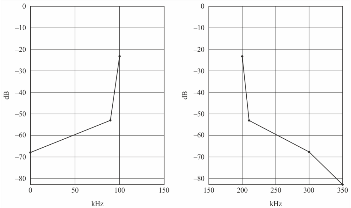
Spectrum mask of spectrum mode F
