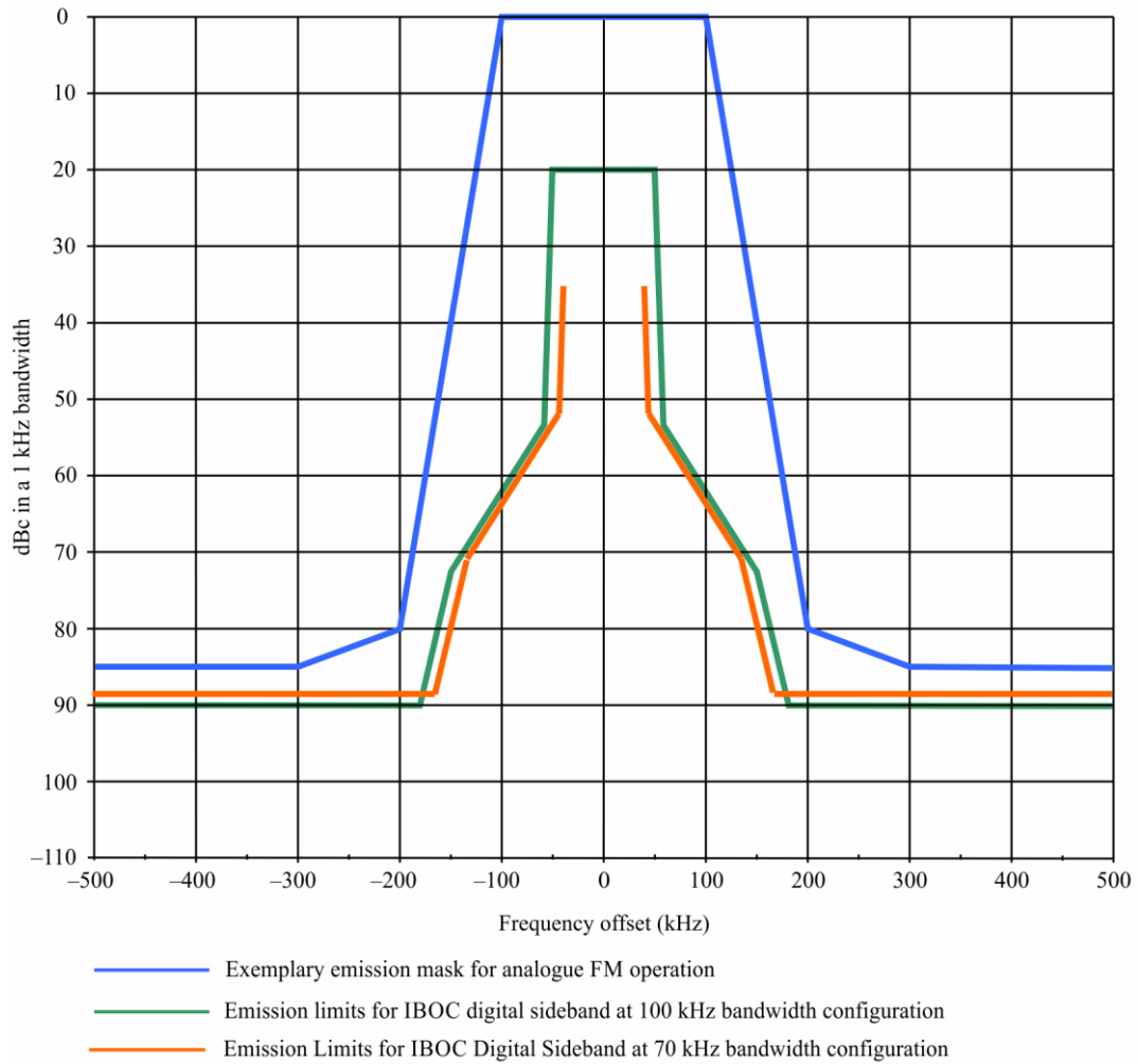
IBOC sideband emission limits*
