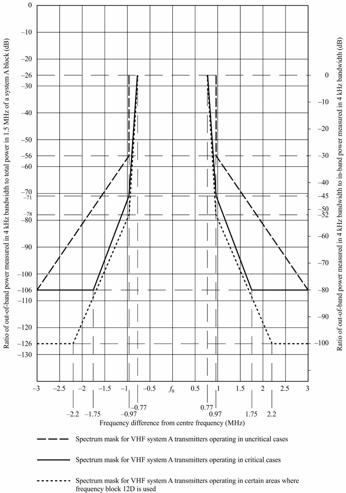
FIGURE 4 Out-of-band spectrum masks for a transmission signal of System A
