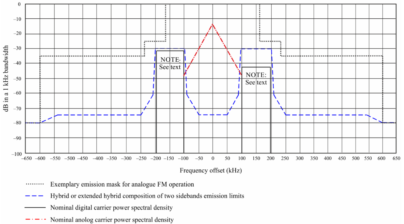
IBOC hybrid mode emission limits*
