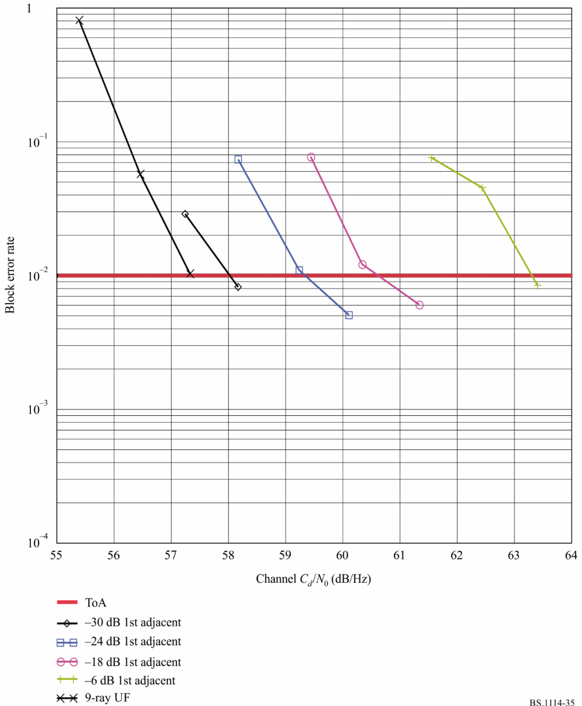
Block error rate results of a hybrid system in 9-ray UF fading with an independently faded first-adjacent interferer
