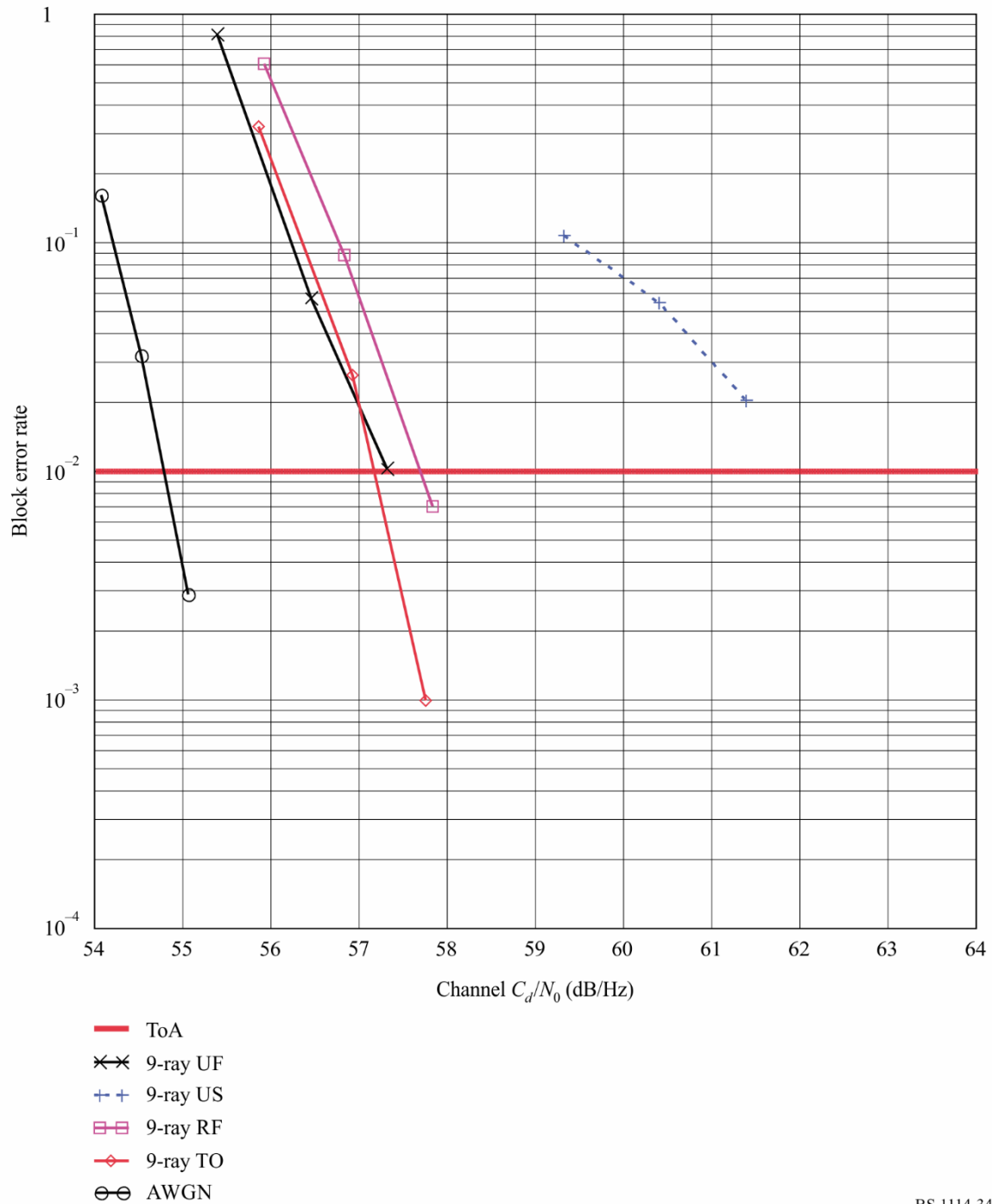
FIGURE 34 Block error rate results of the hybrid system in different types of 9-ray fading and additive white Gaussian noise (AWGN)
