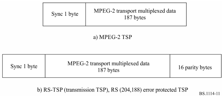
FIGURE 11 MPEG-2 TSP and RS-TSP (transmission TSP)
