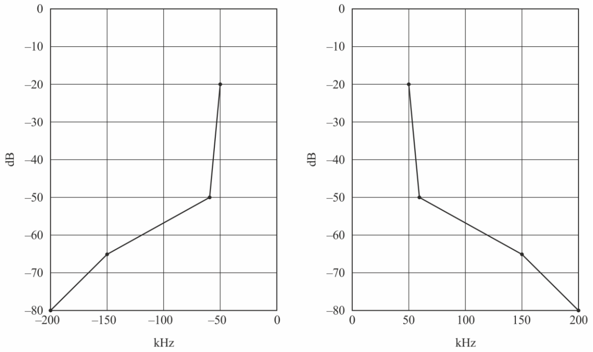
Spectrum mask of spectrum mode A
