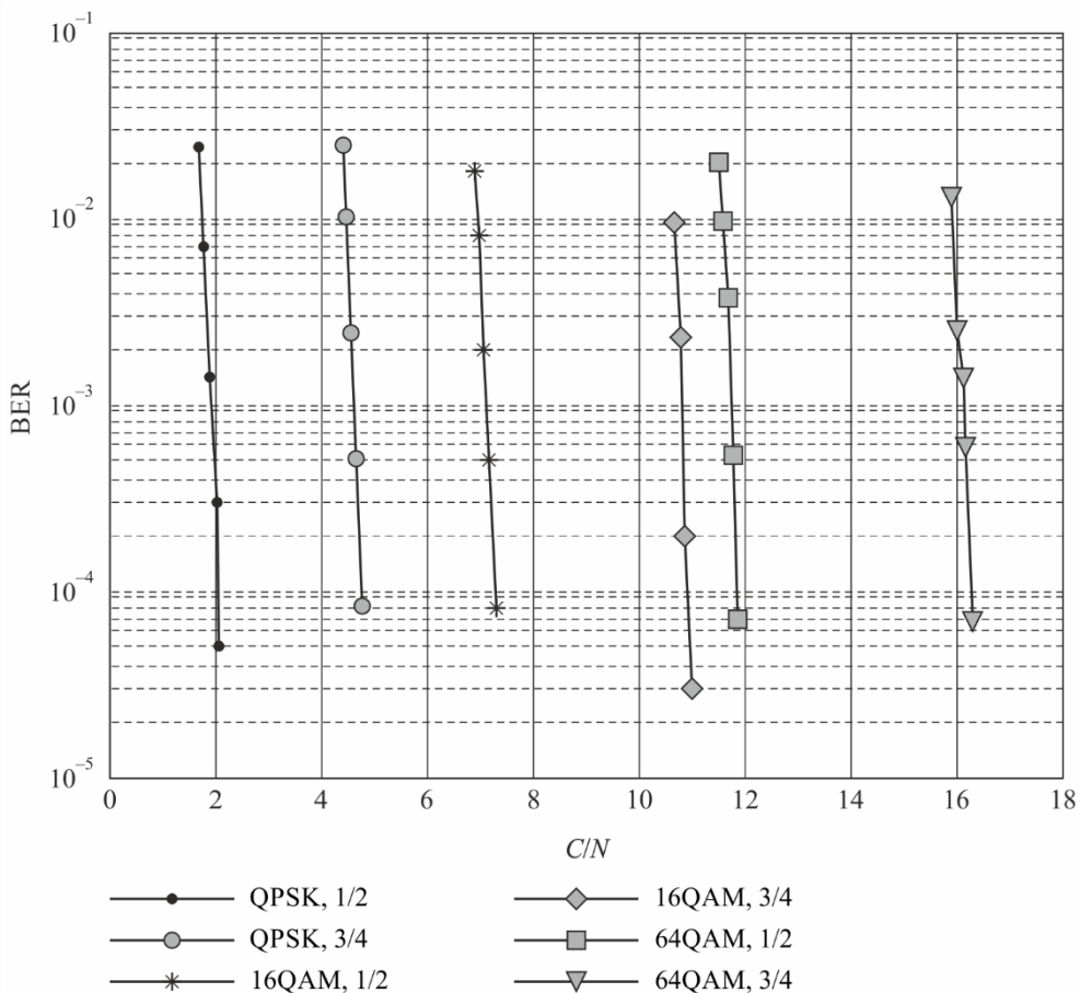
BER vs. C/N in Gaussian channel
