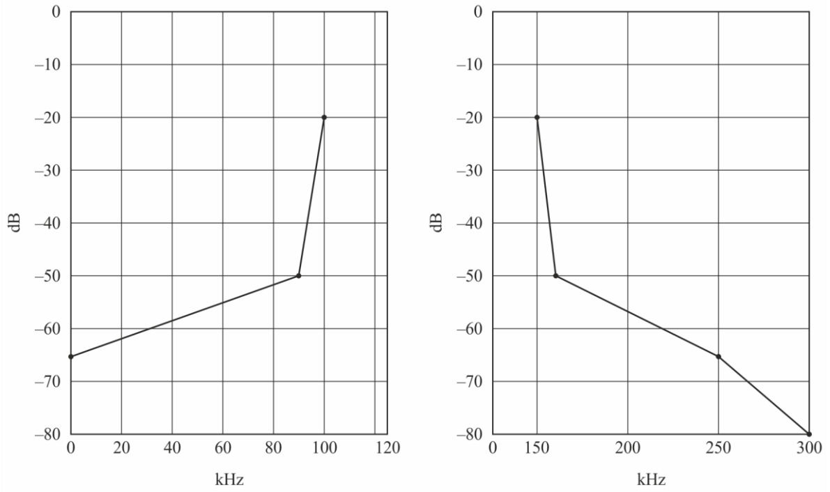
Spectrum mask of spectrum mode E
