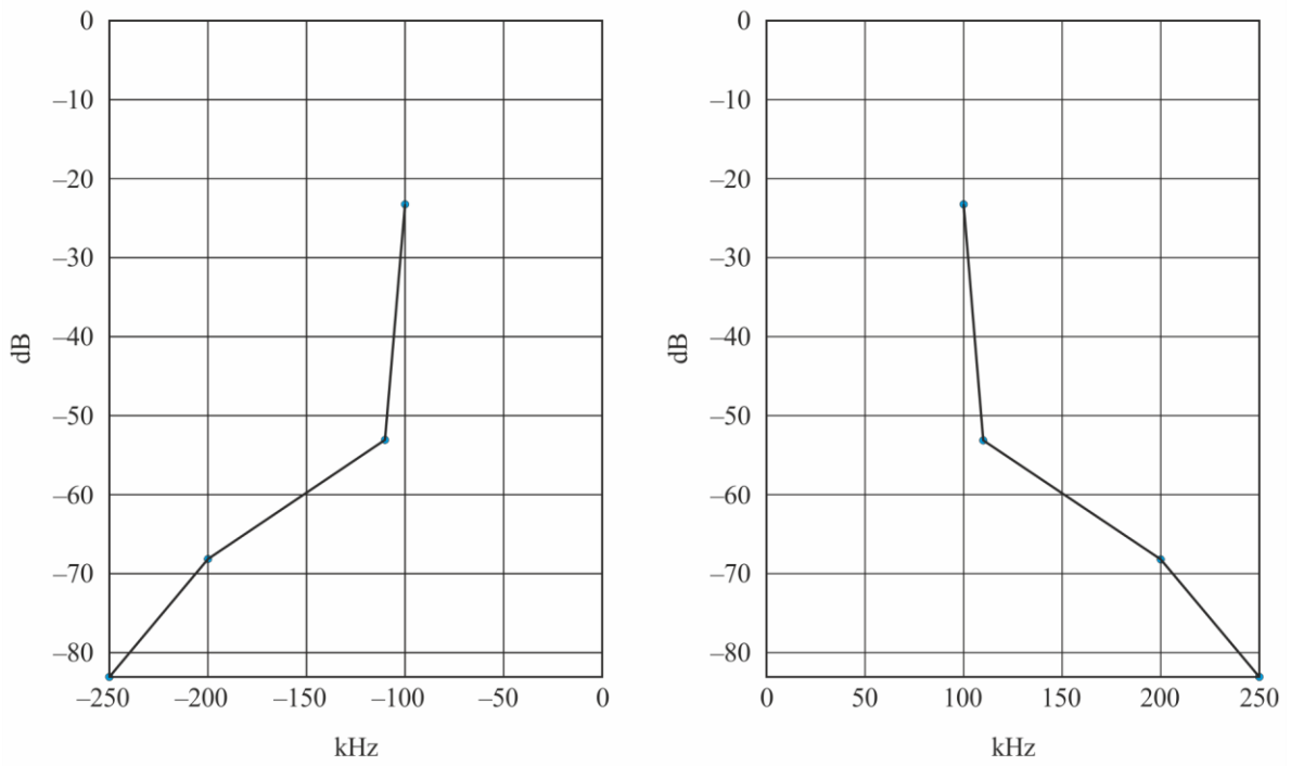
Spectrum mask of spectrum mode B
