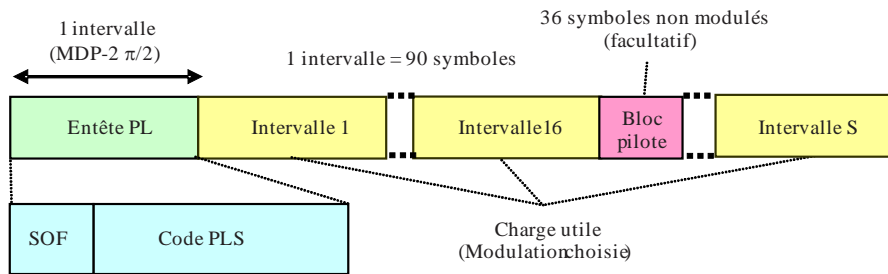
FIGURE 3 Structure de la trame PL
