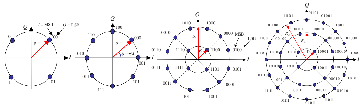
FIGURE 2 The four possible DVB-S2 constellations before physical layer scrambling
