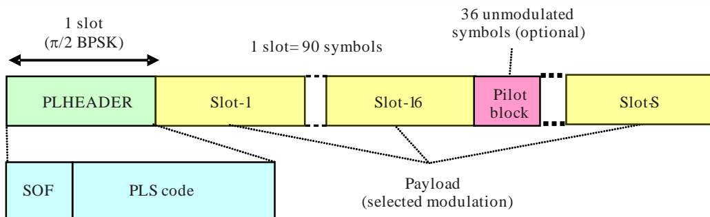
FIGURE 3 PL frame scheme
