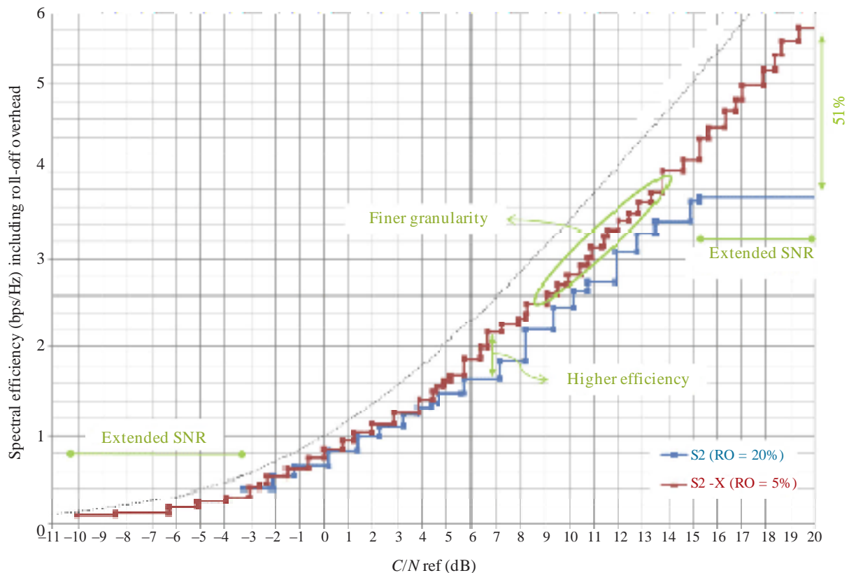
FIGURE 4 Performance comparison of DVB-S2 and DVB-S2X
