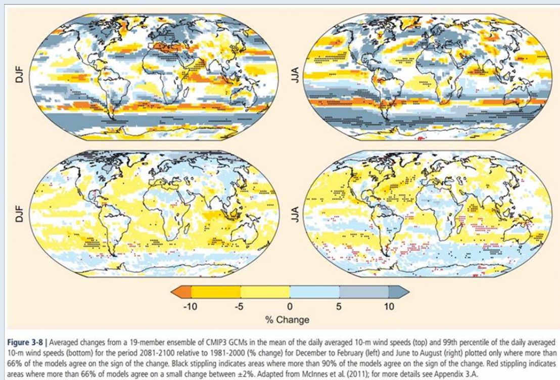
Figure 2: Projected wind speed changes for 2081-2100
