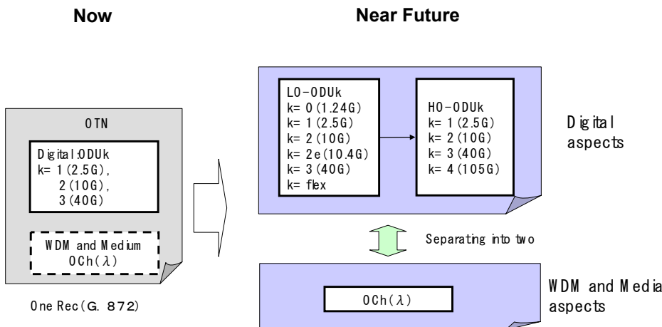
Figure 5-2: Direction of OTN evolution
