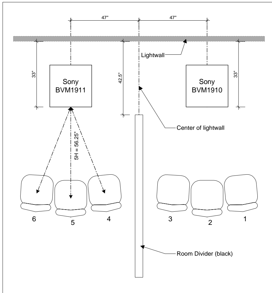
Theatre Setup for VQEG Tests
