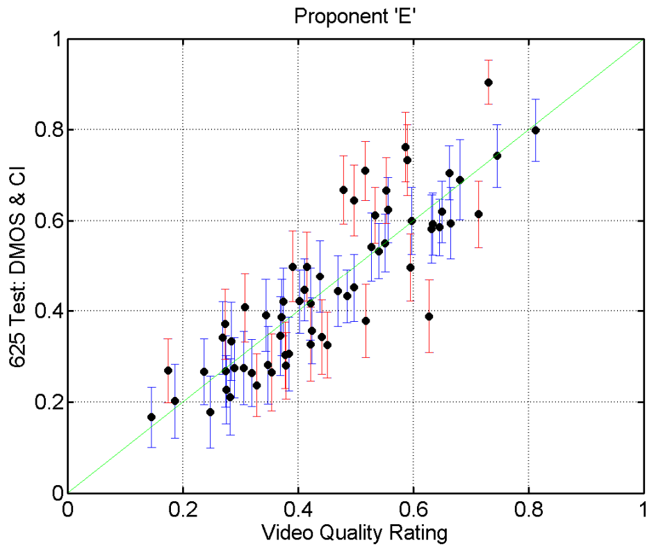
Figure 11 – 625Test – DMOS & CI versus VQR (Proponent 'E')
