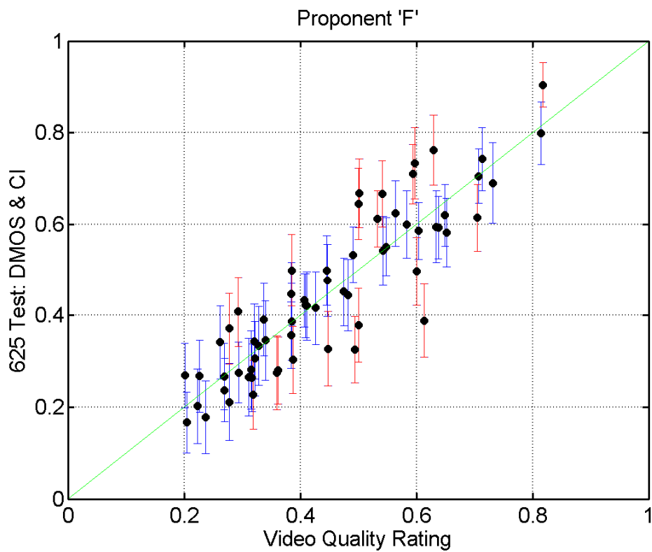
Figure 12 – 625Test – DMOS & CI versus VQR (Proponent 'F')
