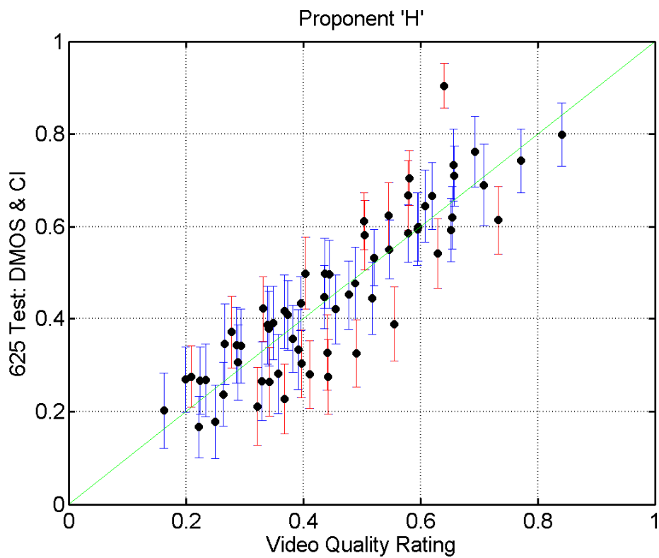
Figure 14 – 625Test – DMOS & CI versus VQR (Proponent 'H')
