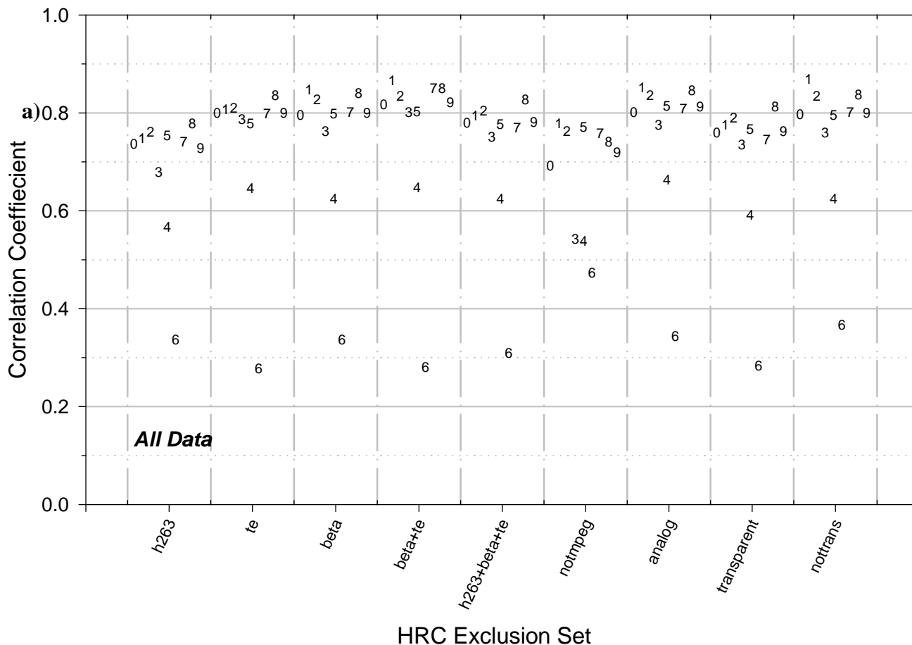
Figure 9 – Non-linear regression correlations computed using all subjective data for the nine HRC exclusion sets
