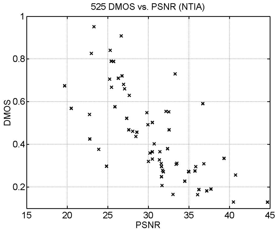
Figure 15 – 525Test – DMOS versus PSNR (results from NTIA)
