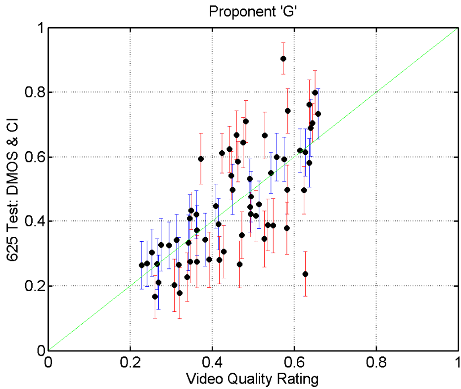
Figure 13 – 625Test – DMOS & CI versus VQR (Proponent 'G')
