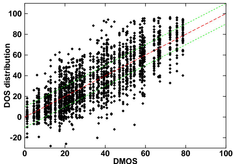
Figure III.4 – Distribution of difference opinion scores corresponding to 525 line videos
