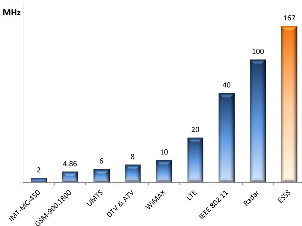
FIGURE 15 Spectrum occupied by radio system (BS) of certain radio technologies, communication modes, system types, MHz
