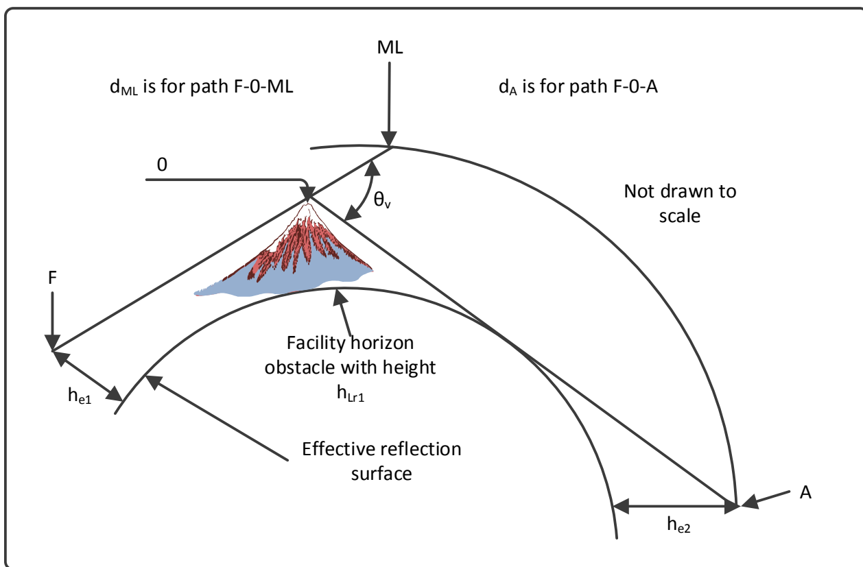
FIGURE 8 Paths used to determine diffraction attenuation
