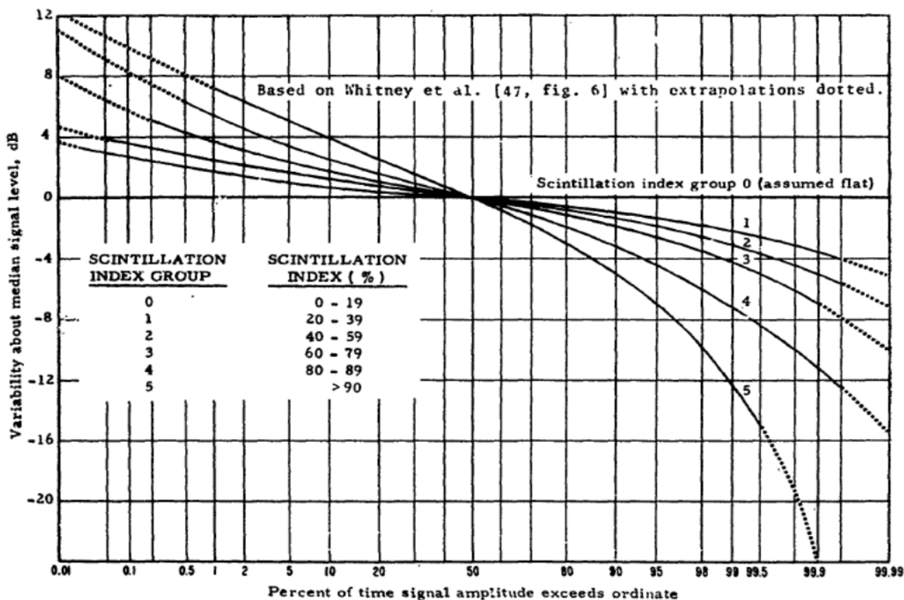
FIGURE 16 Signal level distribution for ionospheric scintillation index groups
