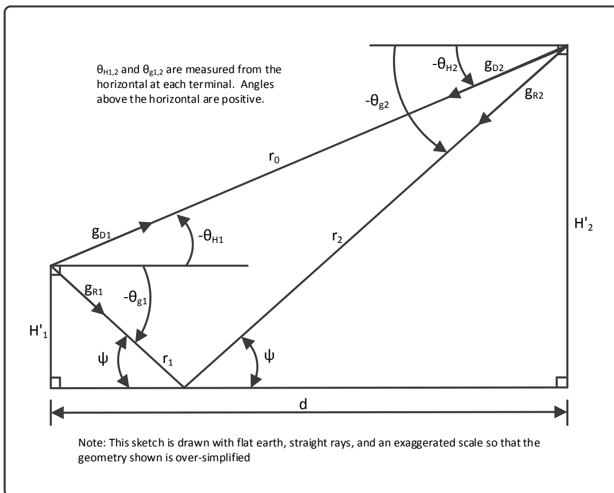
Antenna gain notation and correspondence between ray take-off angles and gains
