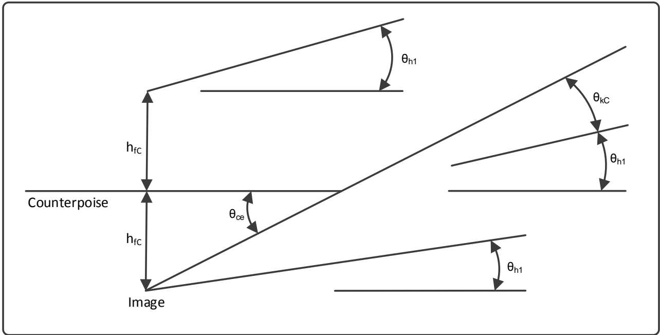
Geometry for earth reflection diffraction parameter, v_c , with limited surface of counterpoise
