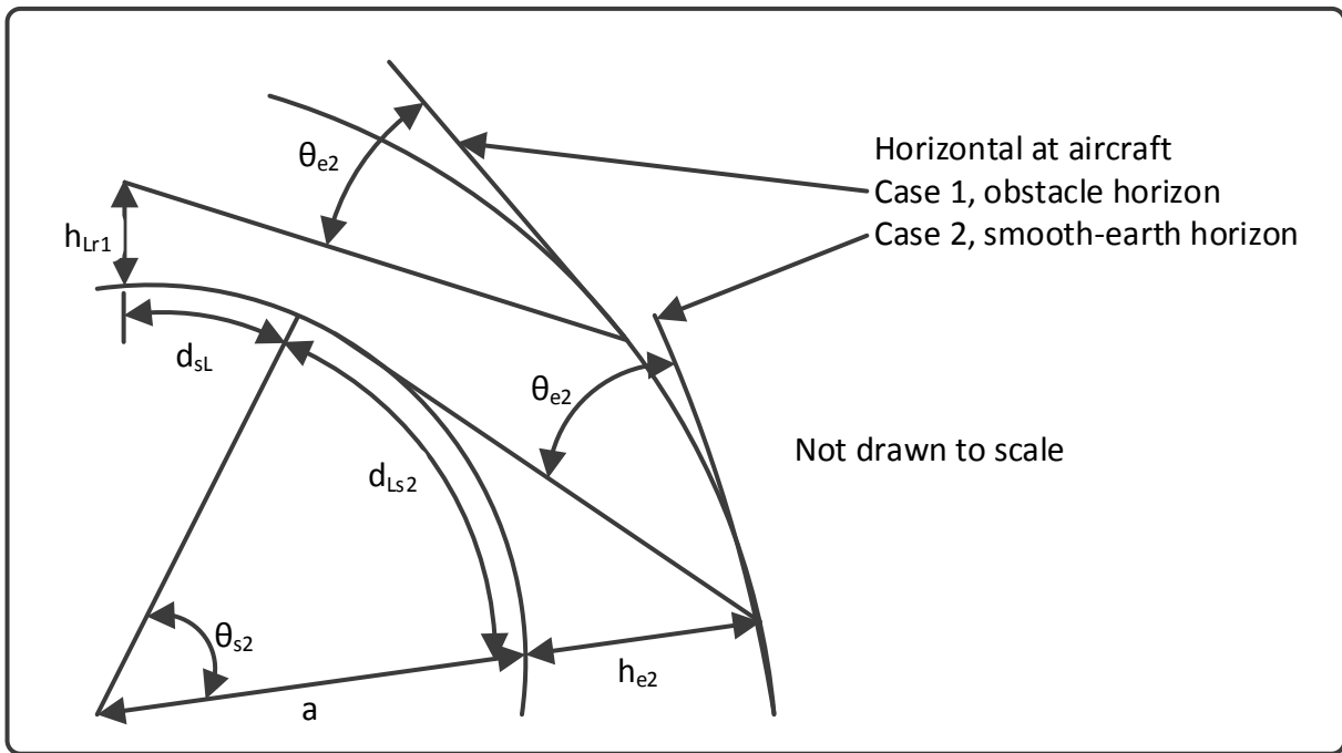
FIGURE 7 Geometry for the higher antenna radio horizon
