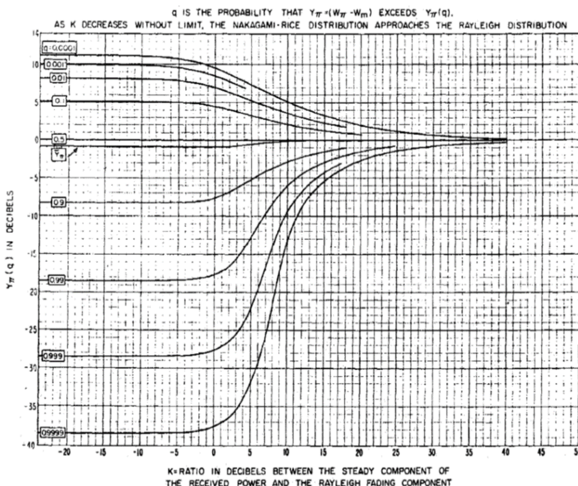
Nakagami-Rice probability distribution of instantaneous fading associated with phase interference [5]
