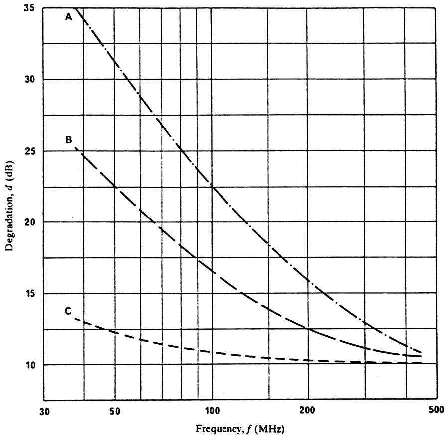
FIGURE 3 – Variation of degradation of mobile reception and minimum values of field strength to be protected for signal quality grade 4 and receiver sensitivity of 0.7 \mu\text{V e.m.f.}
