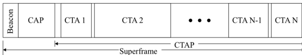
FIGURE 9 802.15.3 superframe
