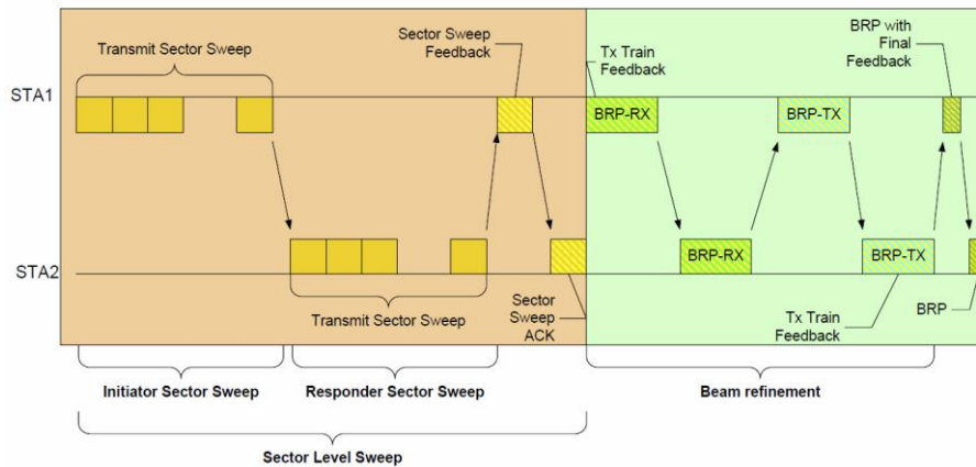
FIGURE 8 Beamforming protocol example
