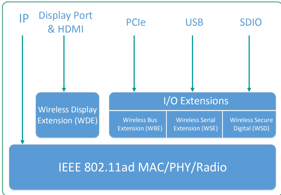
FIGURE 15 WFA WiGig Wireless extensions PALs
