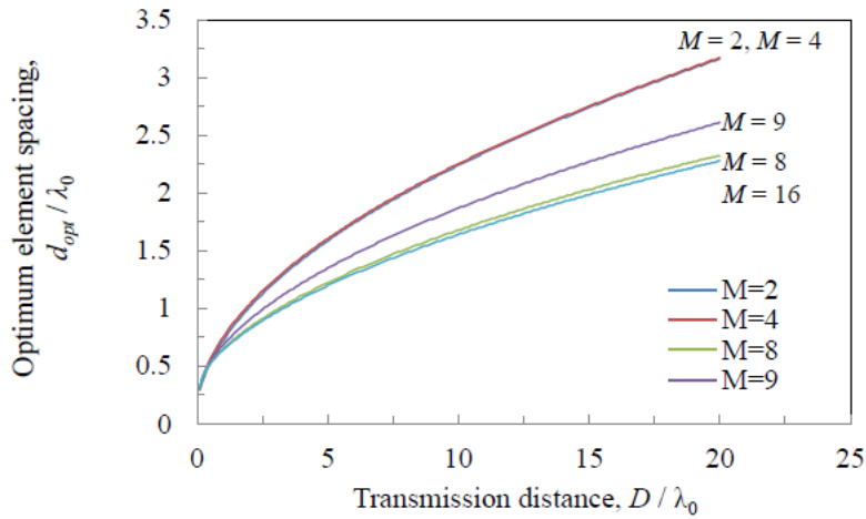
FIGURE 11 Optimum MIMO antenna element spacing
