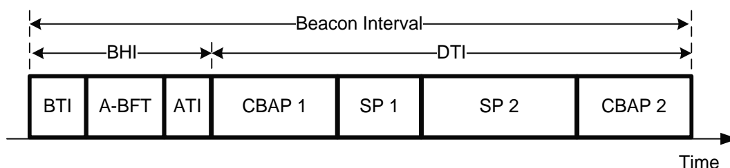
FIGURE 7 Beacon interval structure
