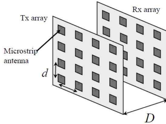
FIGURE 10 Basic structure of MIMO with M=16
