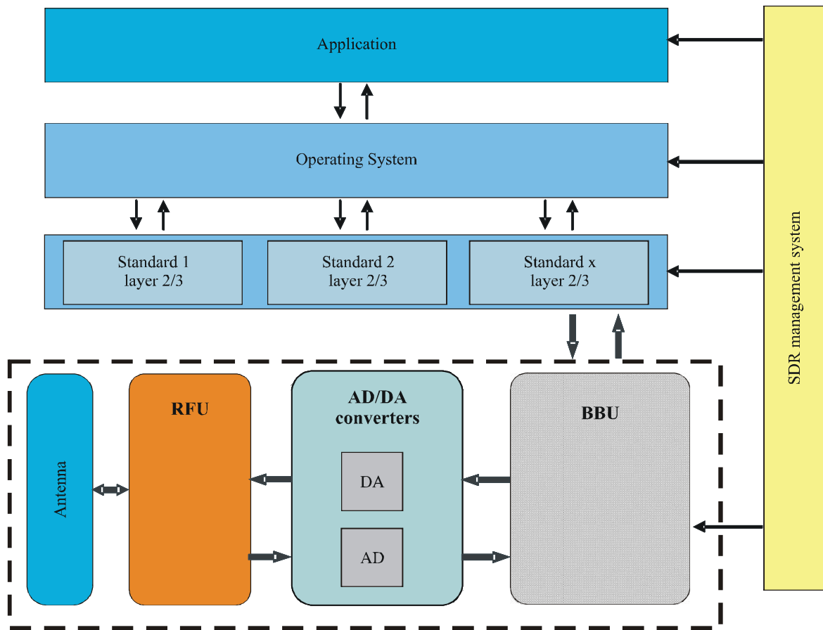
Basic architecture of SDR
