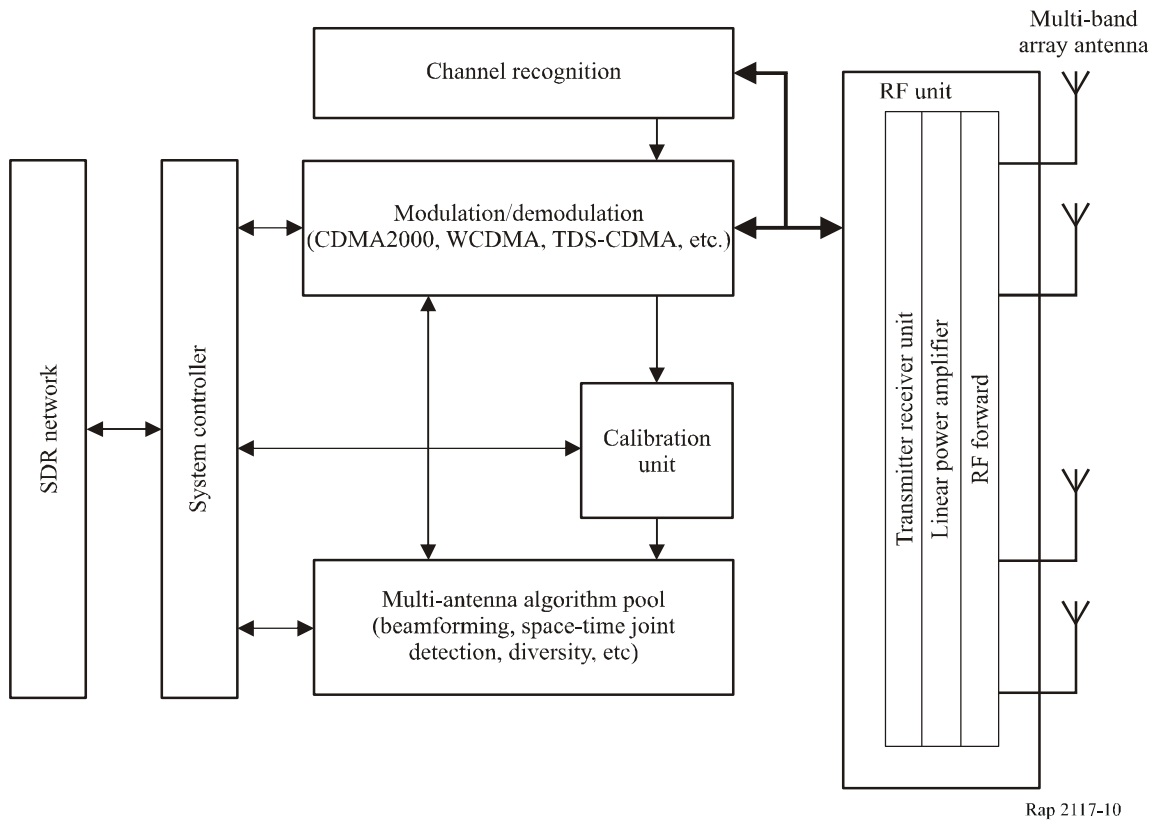
Architecture of software adaptive antenna
