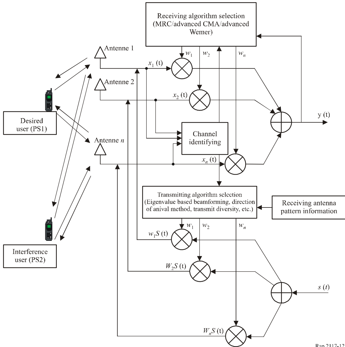
Configuration of software adaptive antenna in TD-SCDMA
