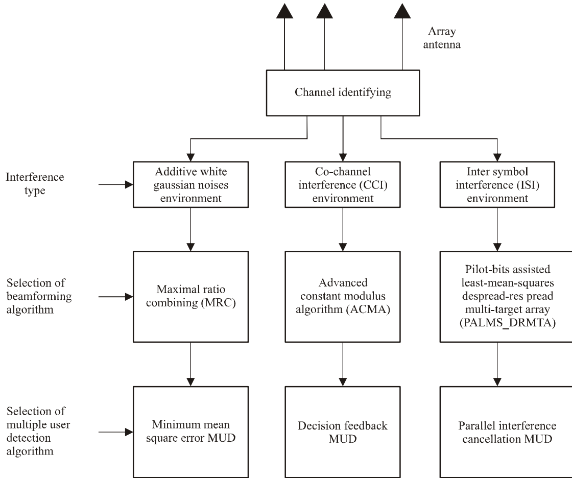
FIGURE 11 Configuration of software adaptive antenna in IMT-2000 CDMA direct spread
