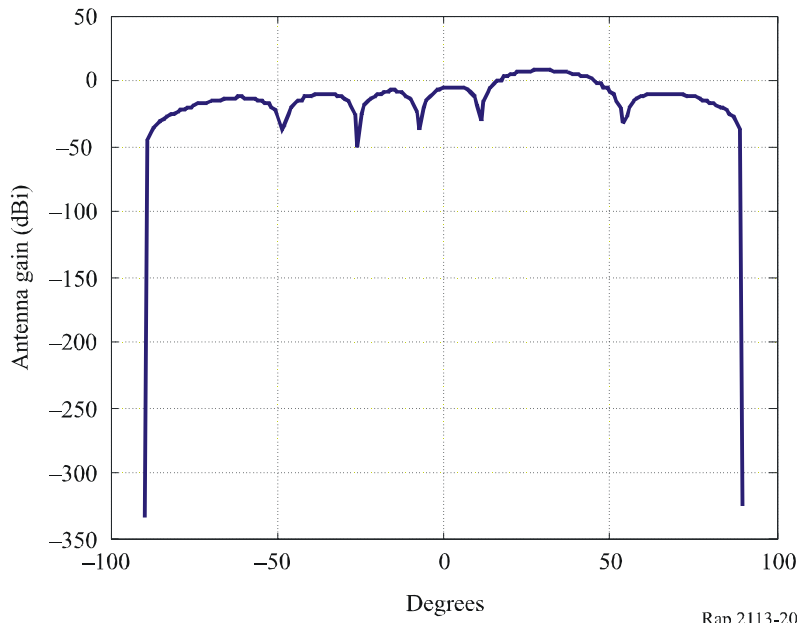
FIGURE 20 Traffic channel 30° smart antenna beam-forming pattern
