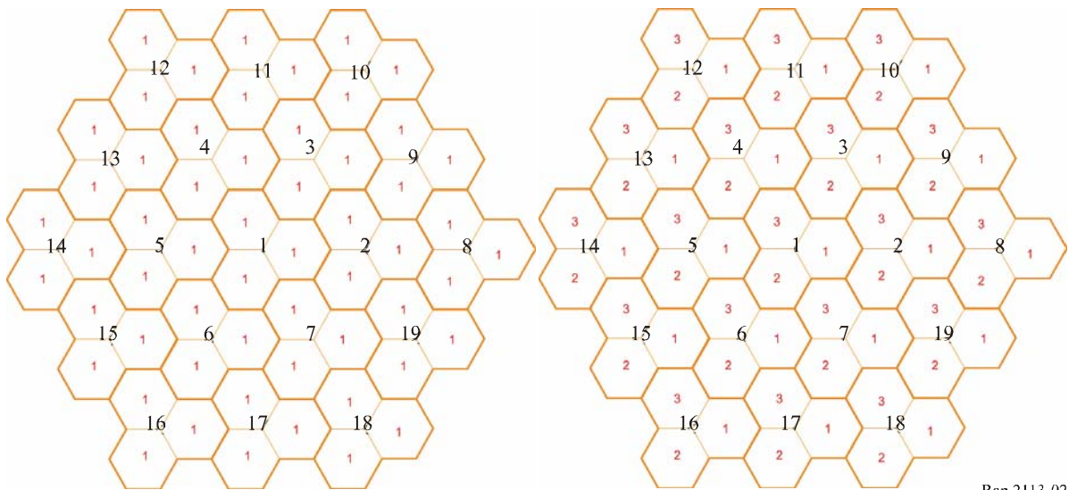
FIGURE 2 802.16 TDD frequency reuse schemes 1 \times 3 \times 1 (left) and 1 \times 3 \times 3 (right)
