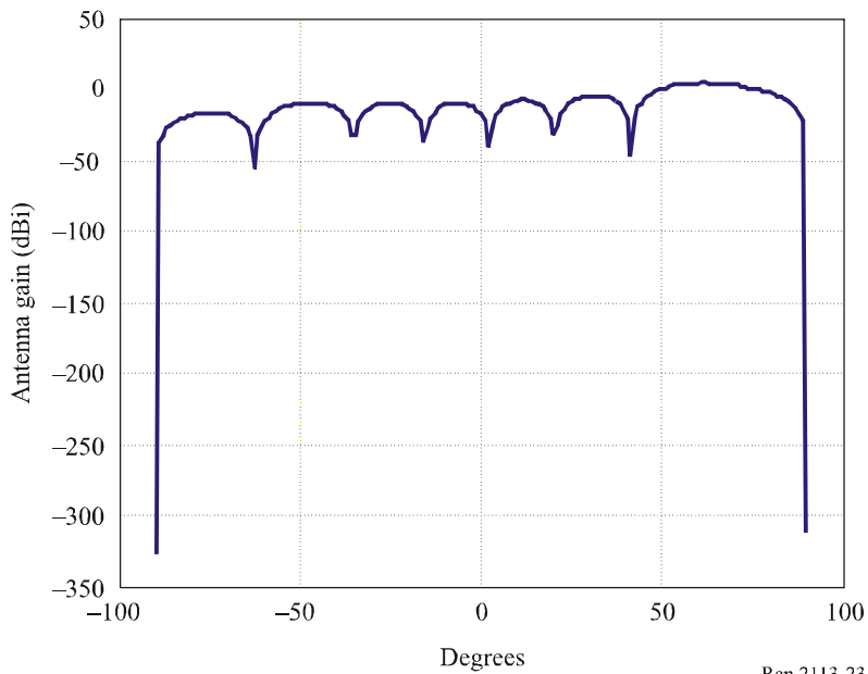
FIGURE 23 Traffic channel 75° smart antenna beam-forming pattern
