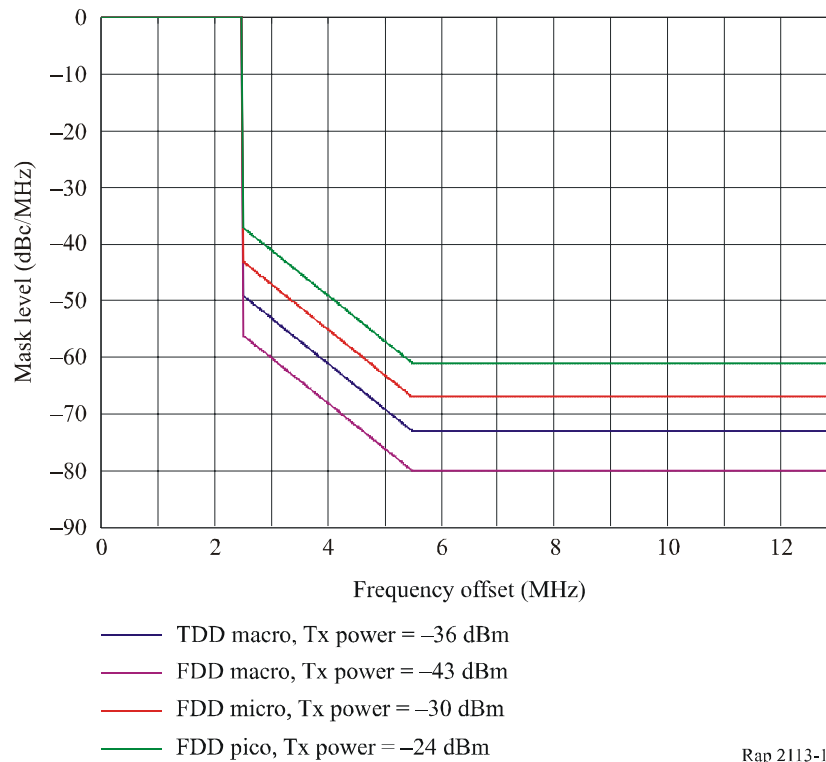
FIGURE 17 FCC spectral mask for 802.16 and FDD base stations
