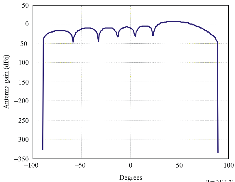
FIGURE 21 Traffic channel 45° smart antenna beam-forming pattern
