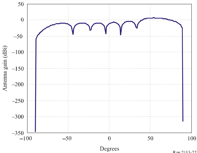
FIGURE 22 Traffic channel 60° smart antenna beam-forming pattern
