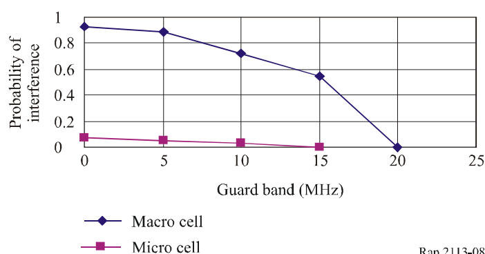
FIGURE 8 Probability of adjacent channel interference from a UMTS base station Transmitter into a MMDS receiver
