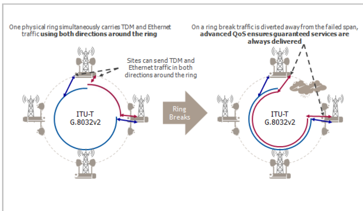
FIGURE 19 ITU-T G.8032v2 networking on a ring break
