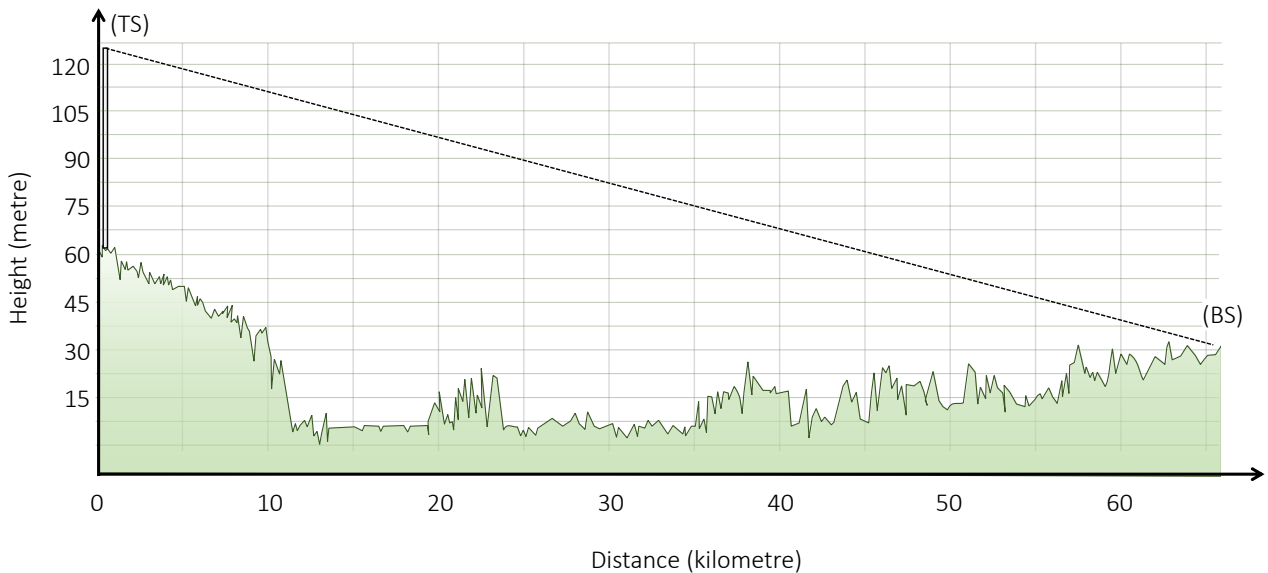
FIGURE 47 Elevation profile, with the distance of approx. 67 km
