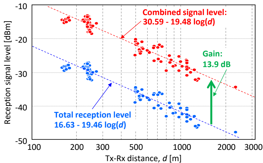
FIGURE 41 Received signal level and diversity gain
