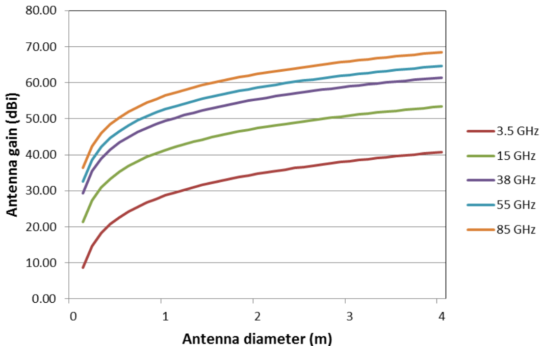
FIGURE 20 Relationship between parabolic antenna gain and antenna diameter ( e_A = 0.55 )
