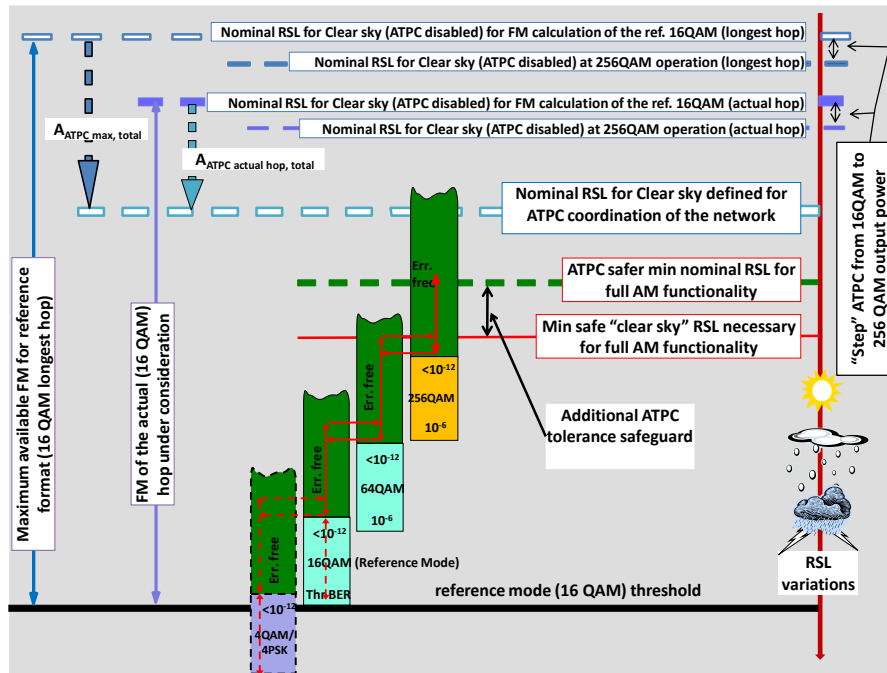
FIGURE 17 Fade Margin and ATPC range impact to adaptive modulation (ECC Report 173)
