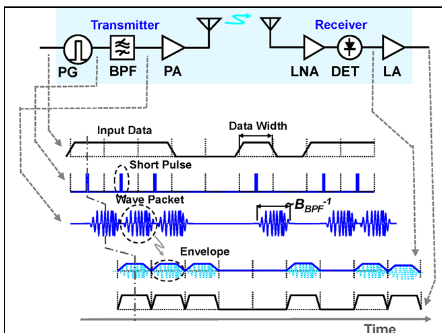
FIGURE 26 Principle of Impulse Radio Technology
