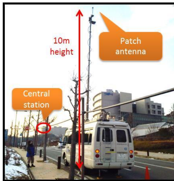
FIGURE 40 Appearance of the mobile base station (Transmitter)
