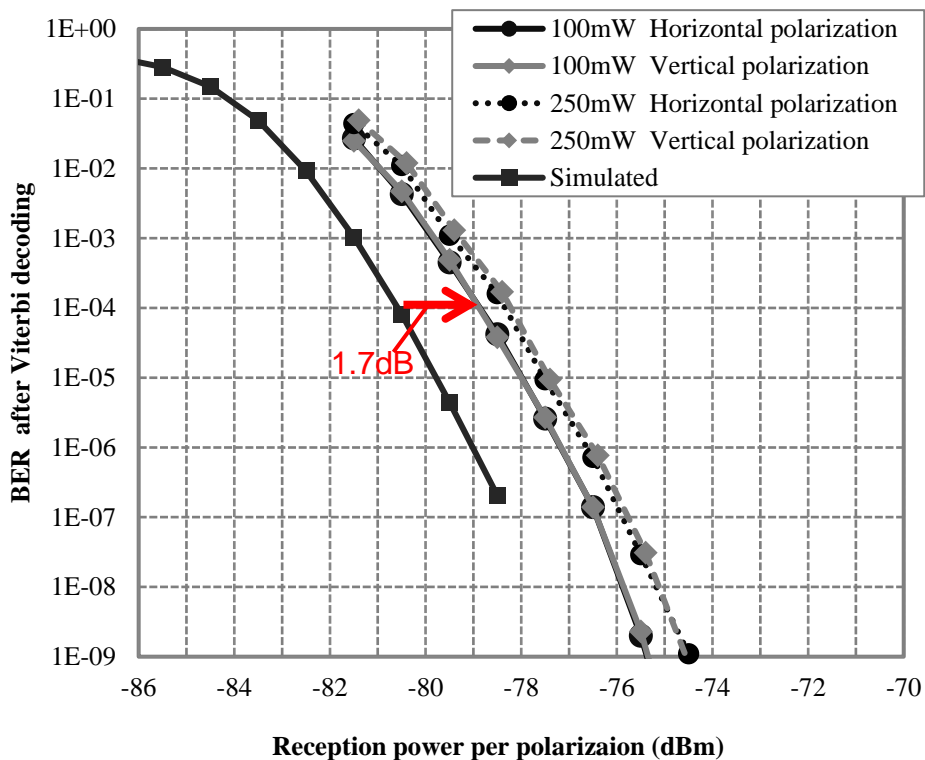
FIGURE 44 BER versus reception power
