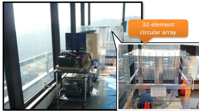
FIGURE 39 Appearance of the central station (Receiver)
