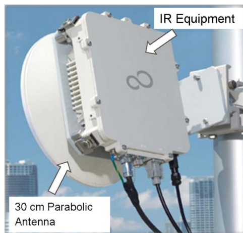
FIGURE 34 Appearance of the equipment using the IR technology
