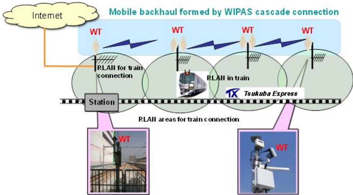
FIGURE 30 Backhaul for Internet access service in moving trains
