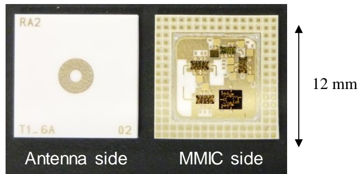
FIGURE 33 Photograph of the antenna/RF module
