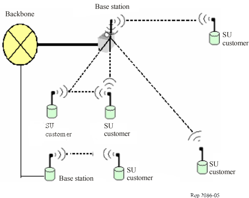
Illustration of network deployment based on combination P-P, P-MP and MP-MP configuration
