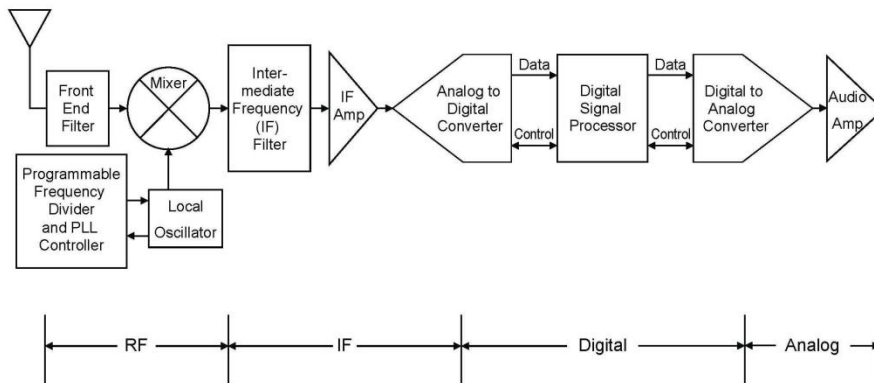
FIGURE 4 Typical frequency-synthesized digital receiver
