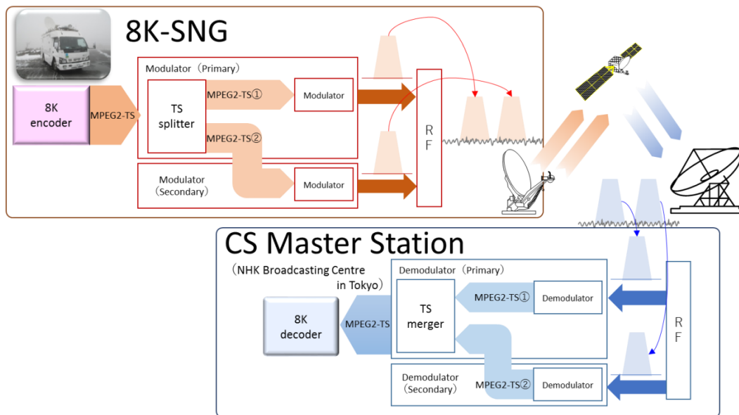
FIGURE 42 Channel bonding
