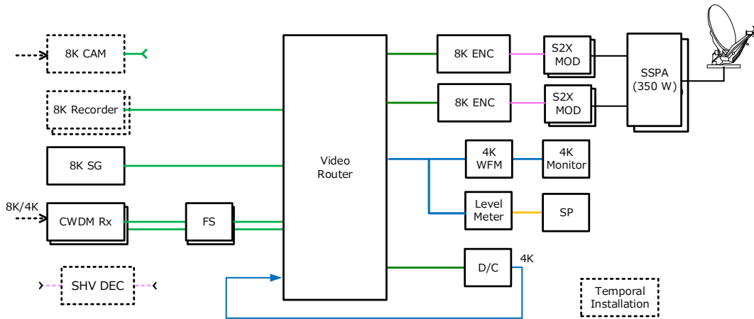
FIGURE 41 Diagram of the video system
