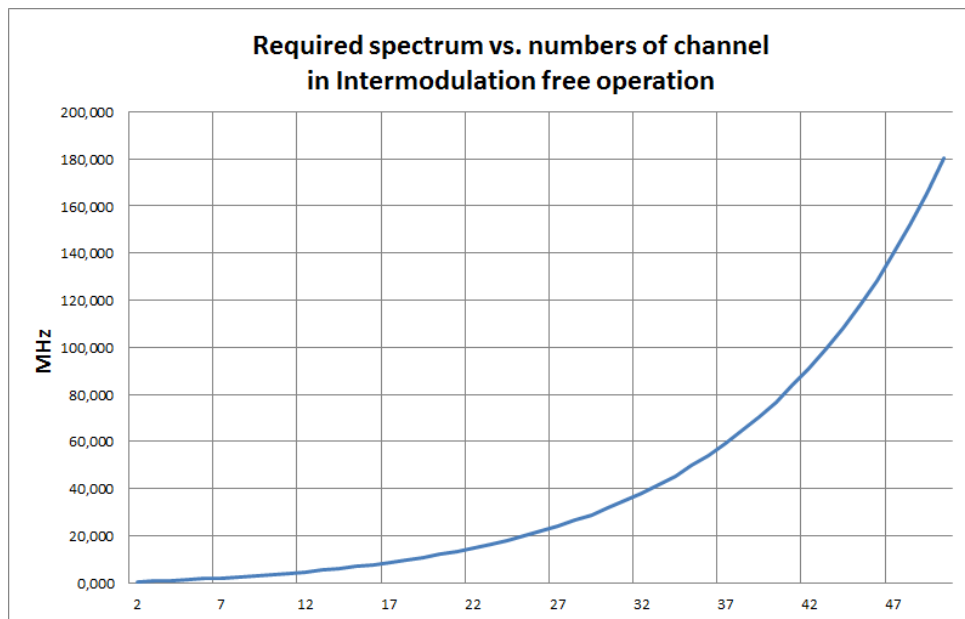
FIGURE 17 Required spectrum vs number of channels in intermodulation free operation for a typical system
