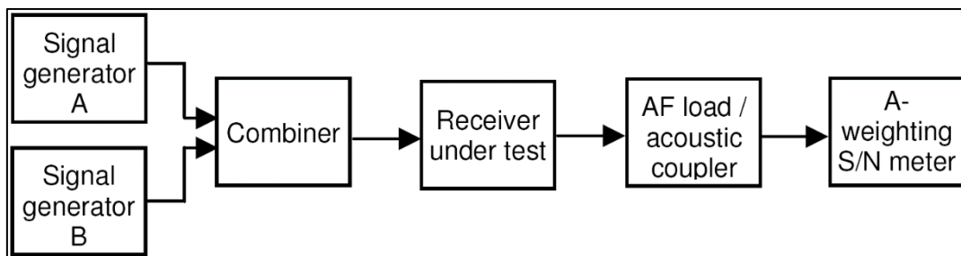
FIGURE 18 Test setup
