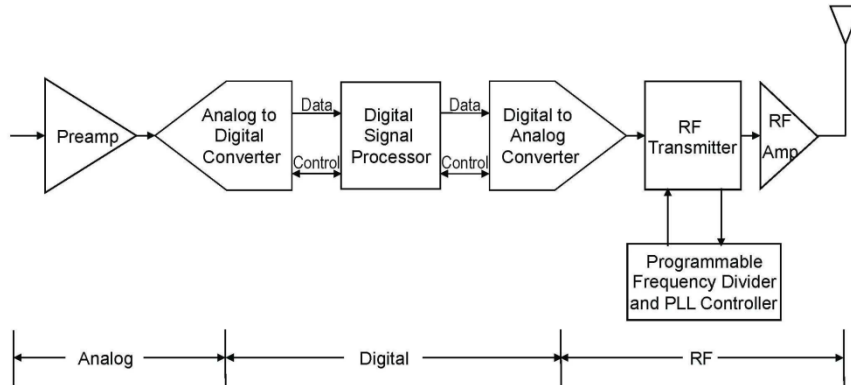
FIGURE 3 Typical frequency-synthesized digital transmitter
