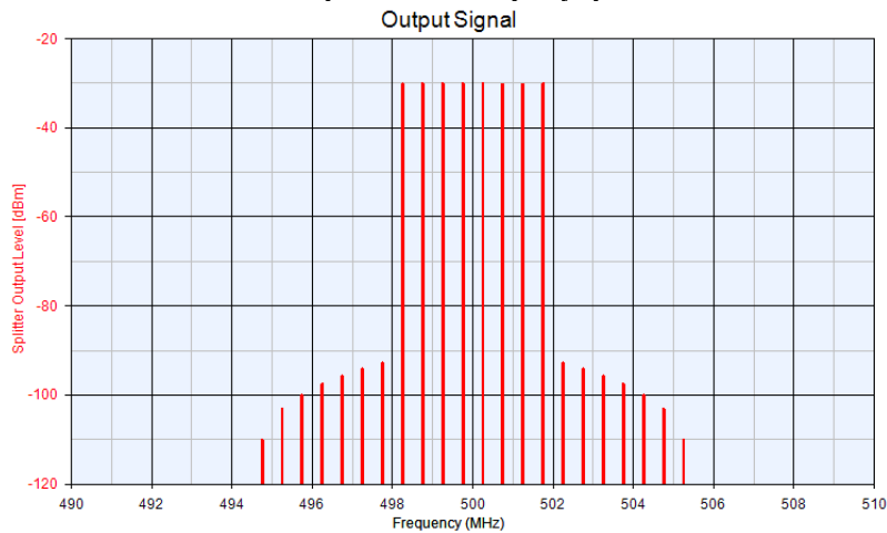
FIGURE 16 Generated intermodulation products for 8 equally spaced transmitter carriers
