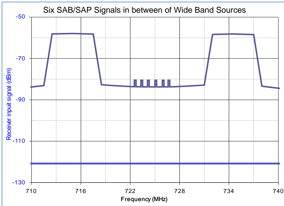
Microphone channel in middle of wideband interferers (Illustration)
