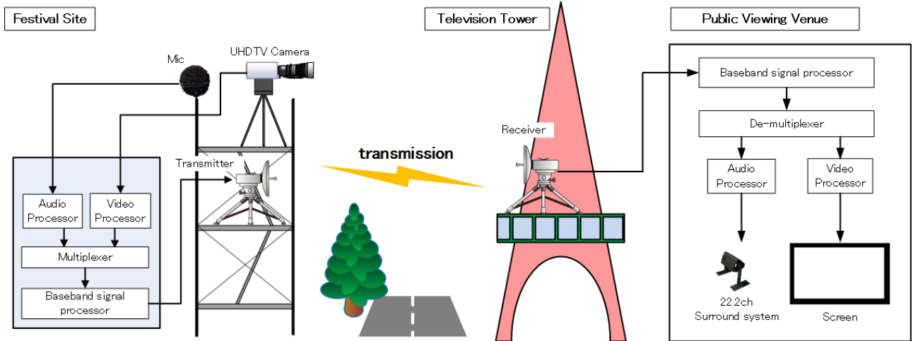
FIGURE 33 System diagram for 8K public viewing
