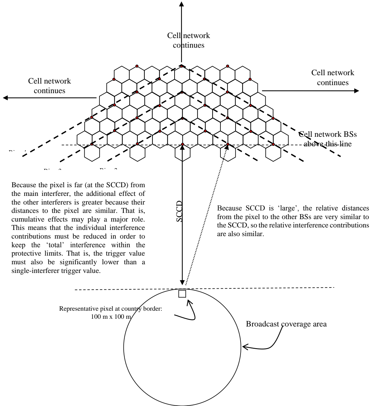
FIGURE 2 Mobile network starts at the 'Single Cell Critical Distance', SCCD, from the border
