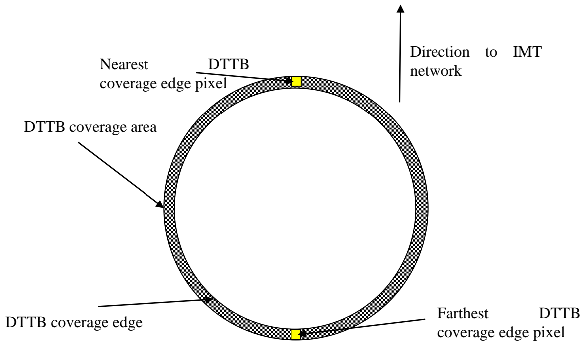
FIGURE 4 DTTB coverage area, coverage edge, nearest and farthest pixels
