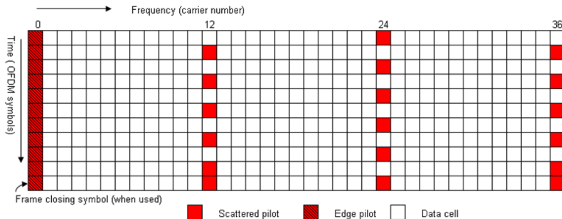
FIGURE A6.3 Scattered pilot pattern PP4 (SISO)
