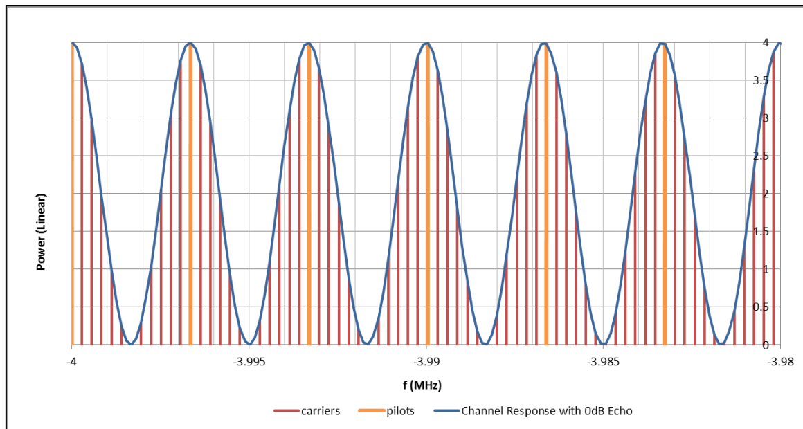
FIGURE A6.5 DTT passband in a perfect channel with 0 dB echo at 300 \mu s delay – linear amplitude
