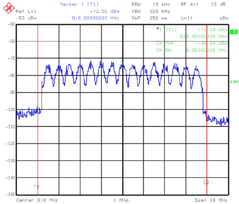
Title: DVB-T signal + single echo (delay = 2us, atten = 5dB) Date: 10.MAY.99 10:30:58
