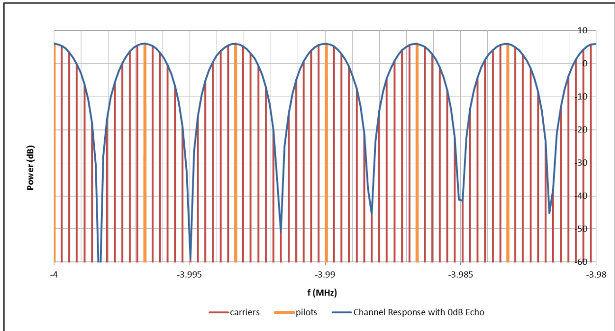
FIGURE A6.4 DTT passband in a perfect channel with 0 dB echo at 300 \mu s delay
