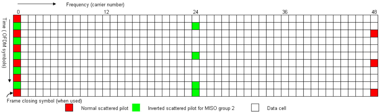
FIGURE 2.9 Pilot pattern 7 – MISO (from [EN 302 755 V1.3.1])
