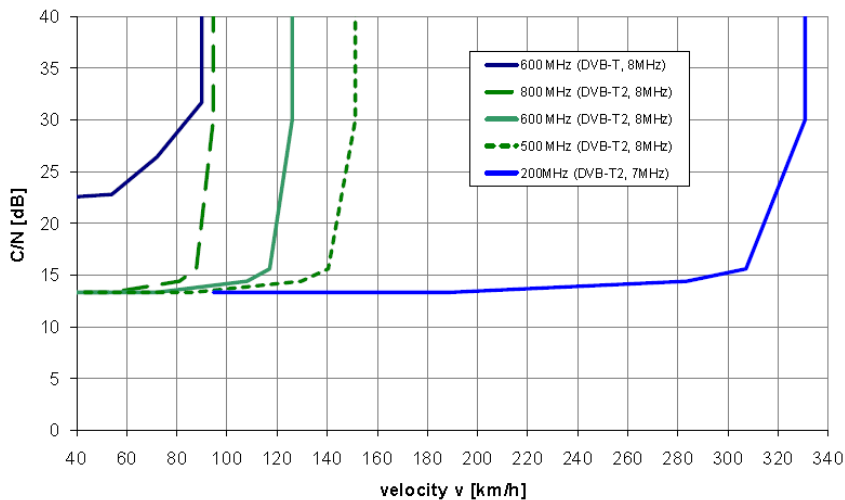
FIGURE 2.10 Required C/N for DVB-T and DVB-T2 as a function of the velocity of the mobile receiver, 8k FFT (from [AFM2010])
