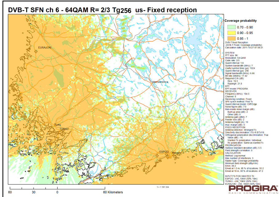
Rooftop reception, SFN, large area, VHF, DVB-T in Finland
