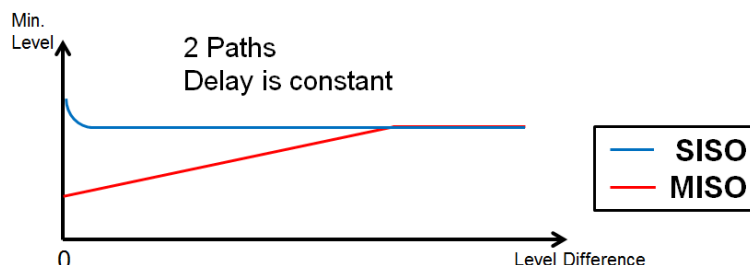
FIGURE 4.12 MISO gain as a function of level difference (MISO gain = difference of min. required levels)
