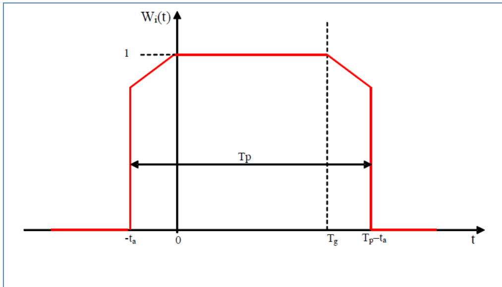
FIGURE A6.1 Weighting function w_i
