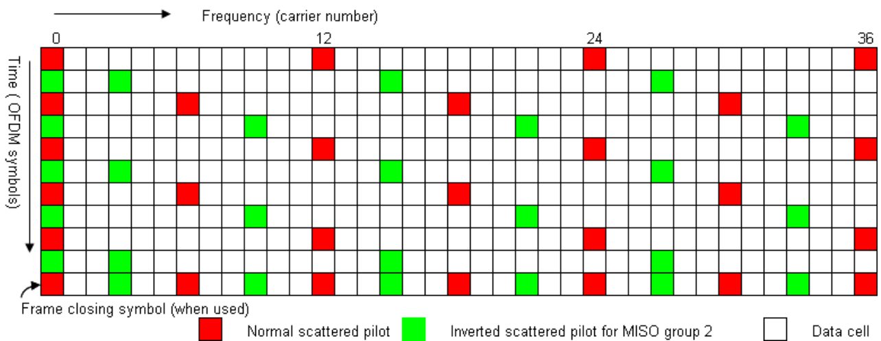
Pilot pattern 1 – MISO (from [EN 302 755 V1.3.1])
