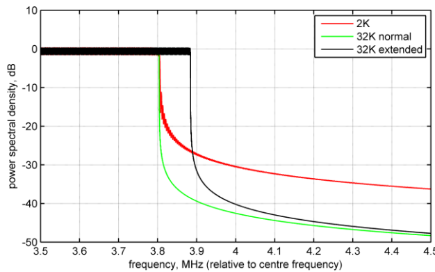
FIGURE 2.12 Detail of theoretical DVB-T2 spectrum for guard-interval fraction 1/8 (for 8 MHz channels) (from [EN 302 755])
