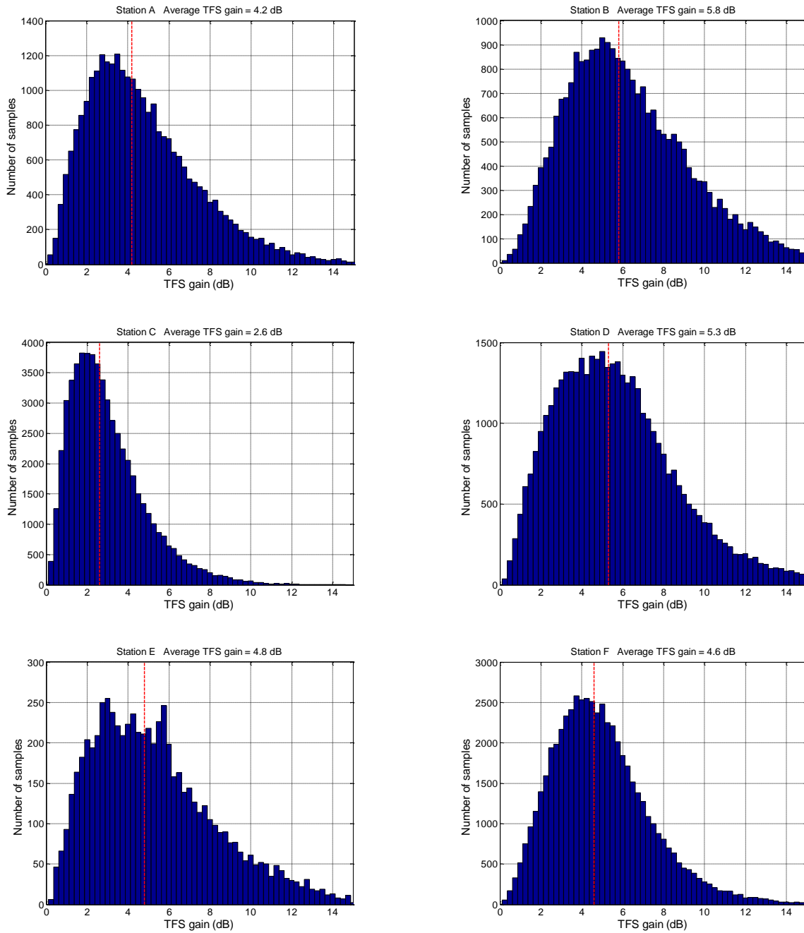
FIGURE 4.18 Measured distribution of TFS gain
