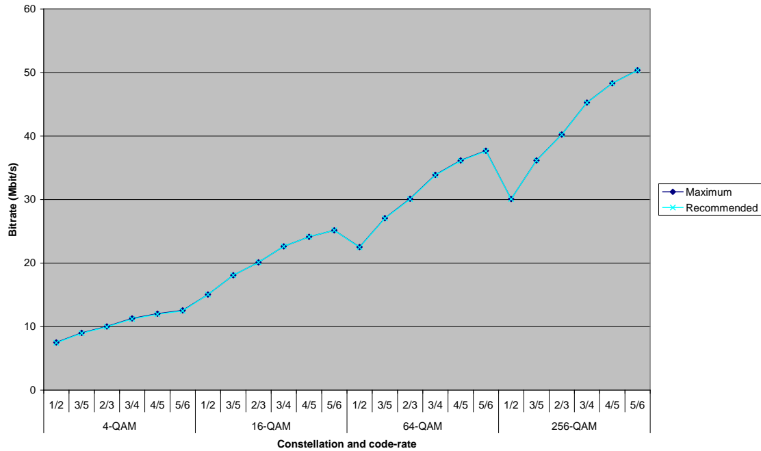
FIGURE 2.1 Maximum bit rate and bit rate for recommended configuration with 8 MHz bandwidth and 32k PP7 (from [TS 102 831])
