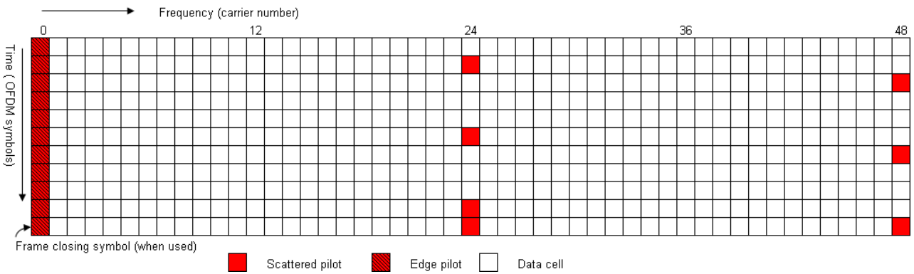
Pilot pattern 7 – SISO (from [EN 302 755 V1.3.1])
