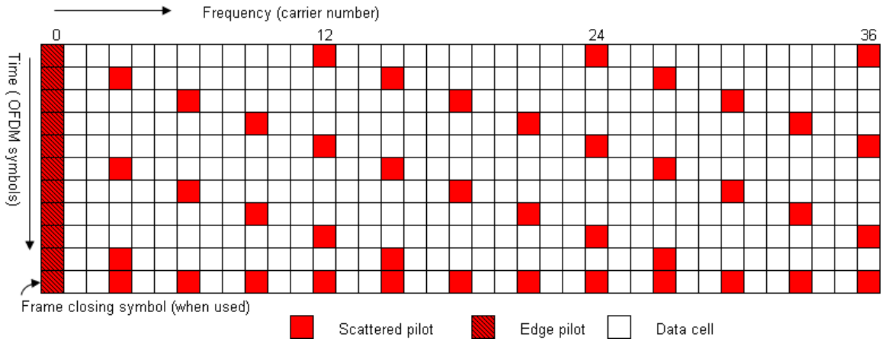
Pilot pattern 1 – SISO (from [EN 302 755 V1.3.1])
