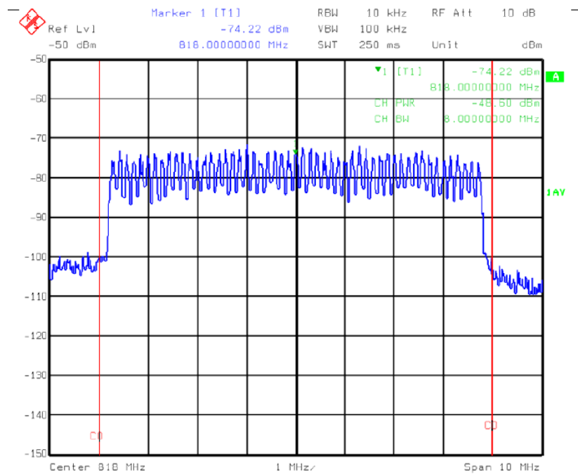
Title: DVB-T signal + single echo (delay = 7us, atten = 5dB) Date: 10.MAY.99 10:27:28
