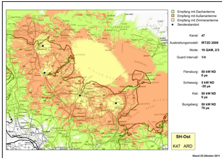
FIGURE 4.5 Portable reception, SFN, medium area, UHF, DVB-T in the northern part of Germany
