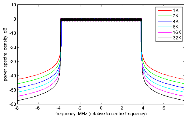
FIGURE 2.11 Theoretical DVB-T2 signal spectrum for guard interval fraction 1/8 (for 8 MHz channels and with extended carrier mode for 8k, 16k and 32k) (from [EN 302 755])
