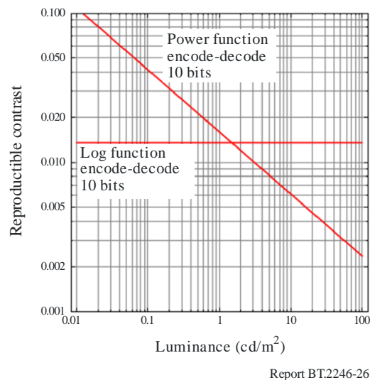
FIGURE 32 Reproducible contrast comparison of log and power functions
