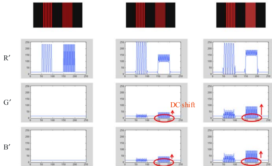
FIGURE 35 Mechanism of clipping in YC transmission
