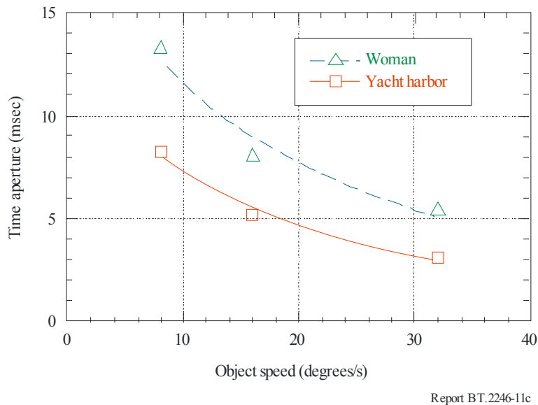
FIGURE 11c Relationship between time aperture and object speed giving an acceptable level of motion blur
