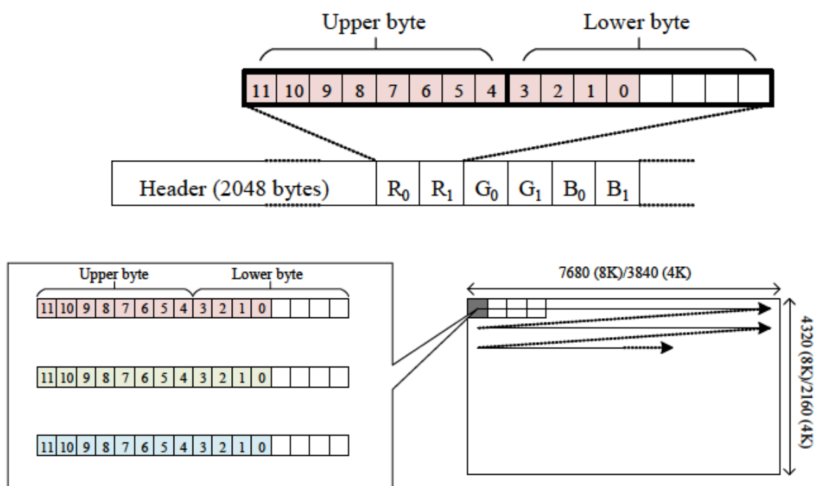
FIGURE 9 Data arrangement for RGB 4:4:4 (12bits)
