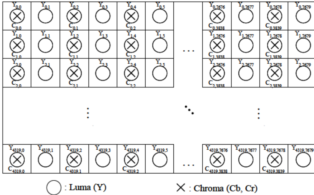
FIGURE 10 Sampling positions in frame
