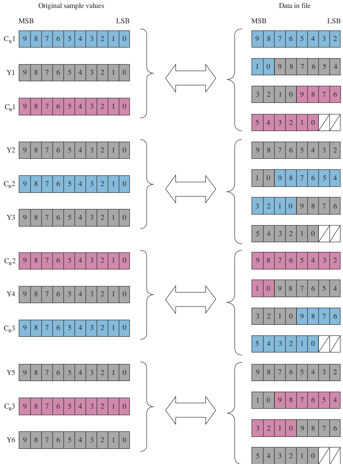
FIGURE 7 Data arrangement for YC B Cr 4:2:2 (10 bits)
