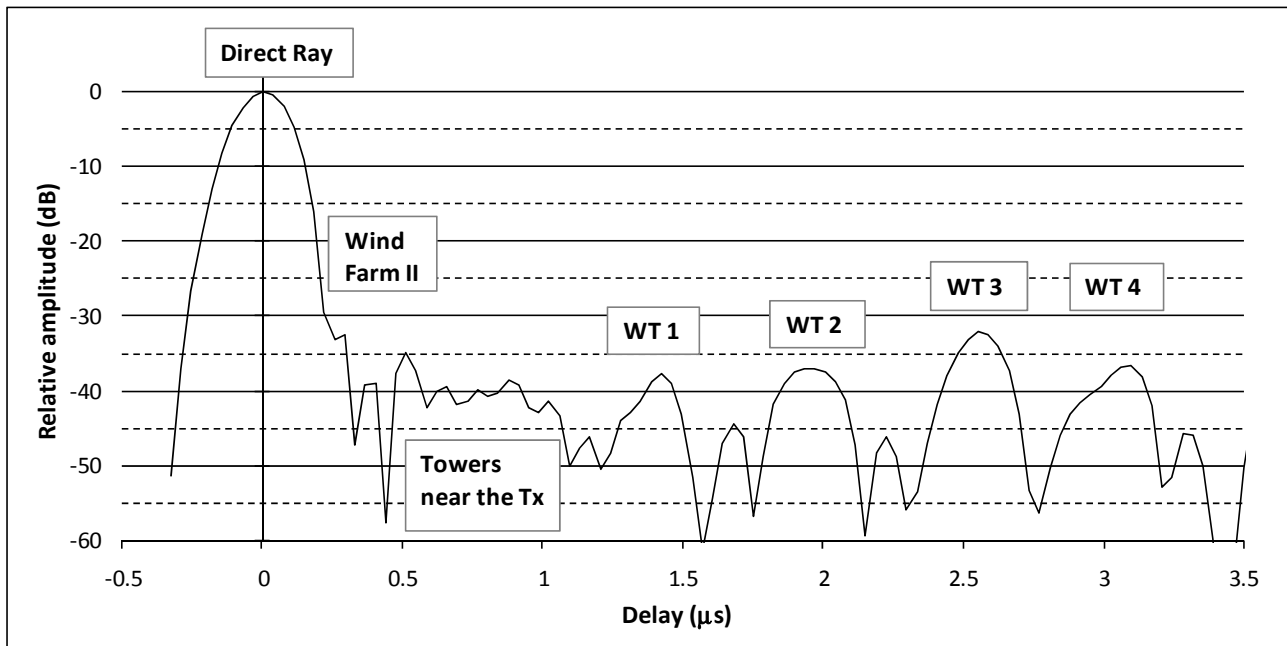
FIGURE 54 Instantaneous DVB-T channel impulse response for static wind turbines
