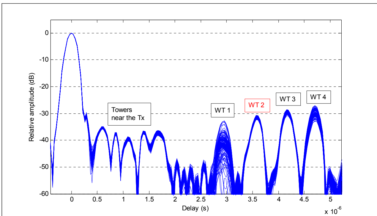
FIGURE 61 DVB-T channel impulse responses recorded during 800 consecutive symbols. Case 2 (Wind farm under normal operation, WT 2 blades are not rotating)
