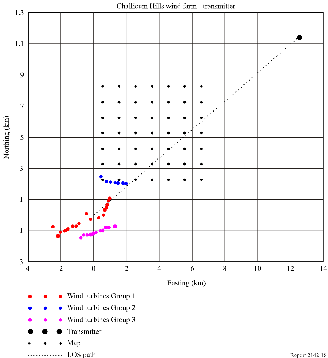
Map of Chalicum wind farm and transmitter location
