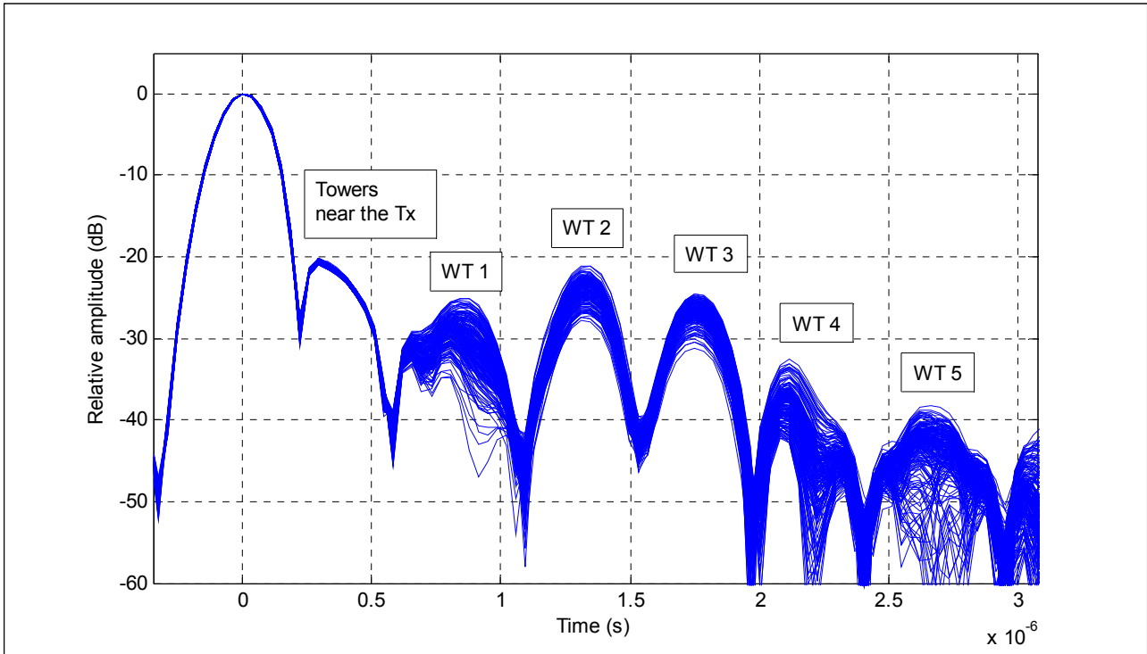
FIGURE 68 DVB-T channel impulse responses during 800 consecutive symbols ( C/N threshold = 19 dB)
