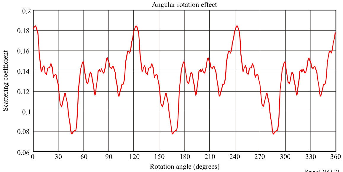
Calculated scattering coefficient variation from 35 turbines for the period of one rotation of the rotor
