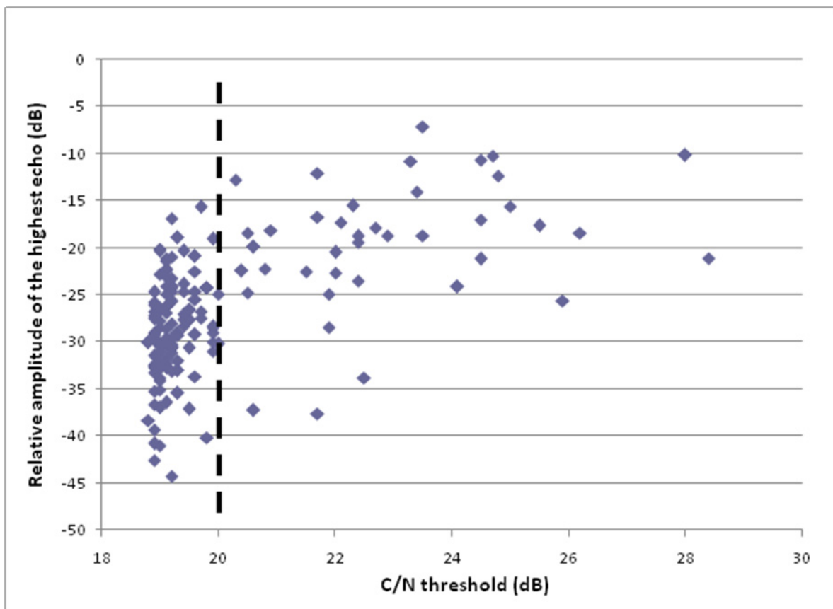
FIGURE 70 C/N threshold ratio as a function of the amplitude of the highest echo
