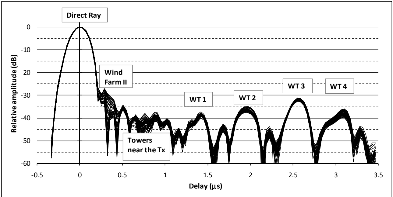
FIGURE 55 DVB-T channel impulse responses for static wind turbines during 200 consecutive symbols
