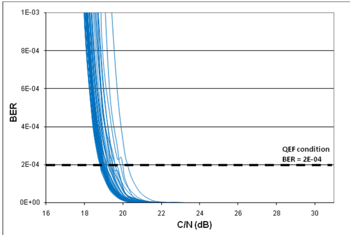
FIGURE 71 Forward scattering: BER after Viterbi as a function of C/N
