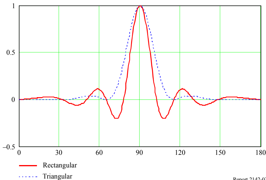
FIGURE 3 Relative scattering patterns (as a ratio) for rectangular and triangular blades. The blade base width is 2.35 m with the incident signal normal to the blade. Frequency = 600 MHz
