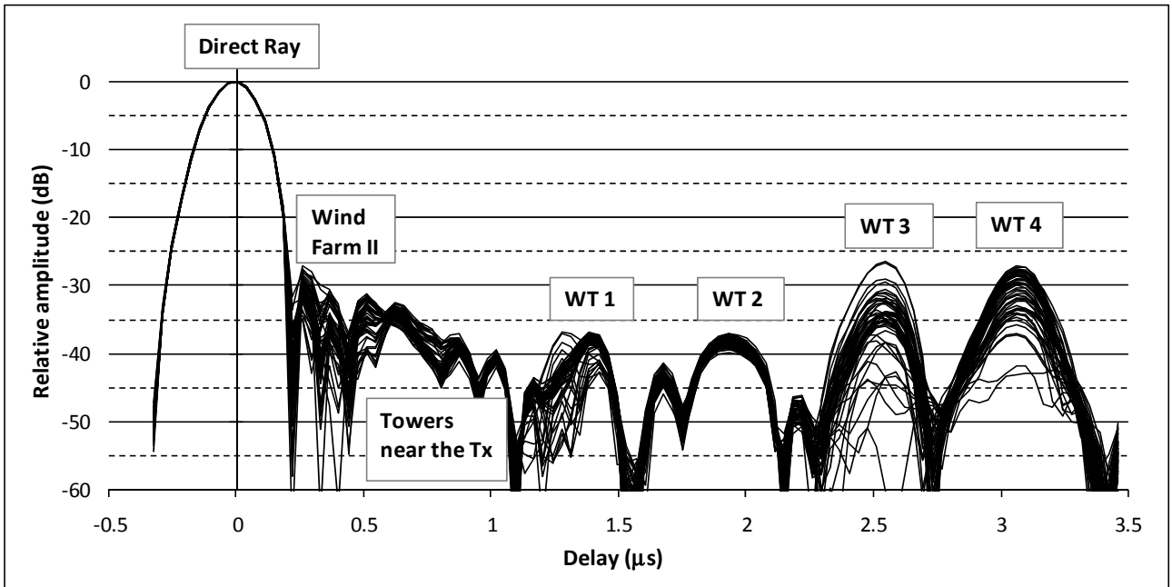
FIGURE 56 DVB-T channel impulse responses recorded during 200 consecutive symbols. All the wind turbines were rotating, while WT 2 was forced to stop
