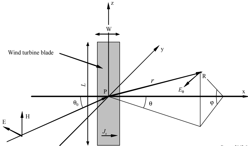
Geometry of wind turbine blade (rectangular, vertical) and incident and scattered signals
