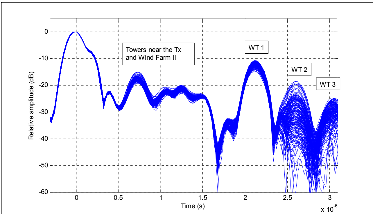
FIGURE 69 DVB-T channel impulse responses during 800 consecutive symbols ( C/N threshold = 24.5 dB)
