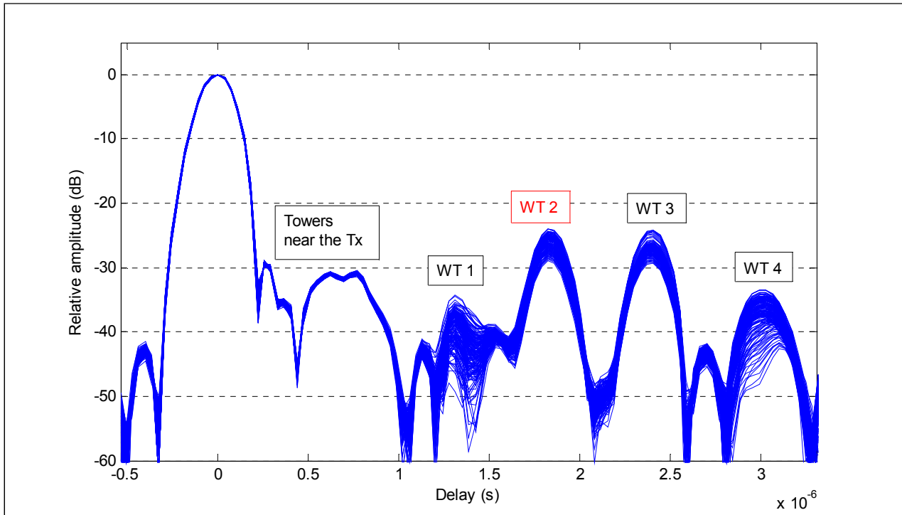
FIGURE 58 DVB-T channel impulse responses recorded during 800 consecutive symbols. Case 1 (Wind farm under normal operation)
