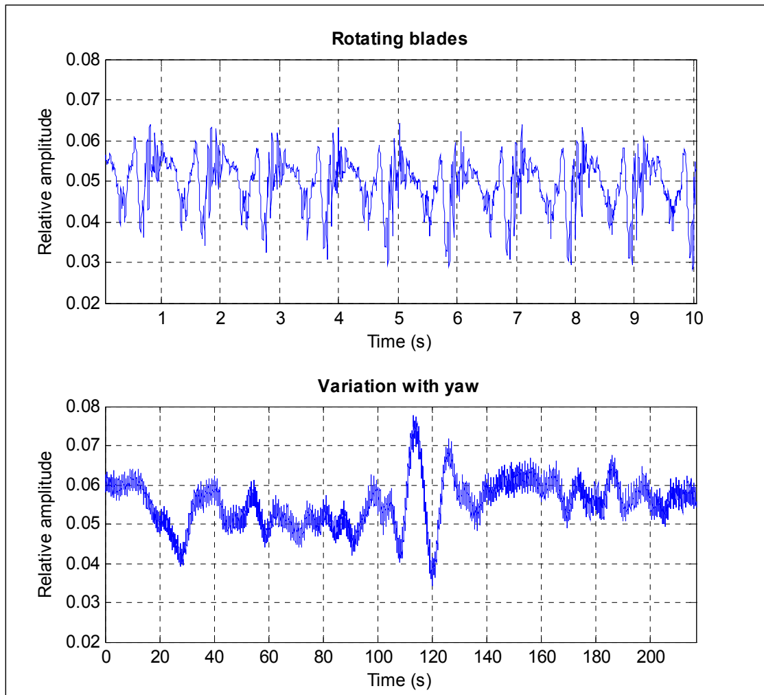
FIGURE 64 Yaw control measurement (Case 1). Comparison between the relative amplitude of the signal scattered by WT 2 under normal operation (above) and during yaw variation (below). Note that different time scale is used
