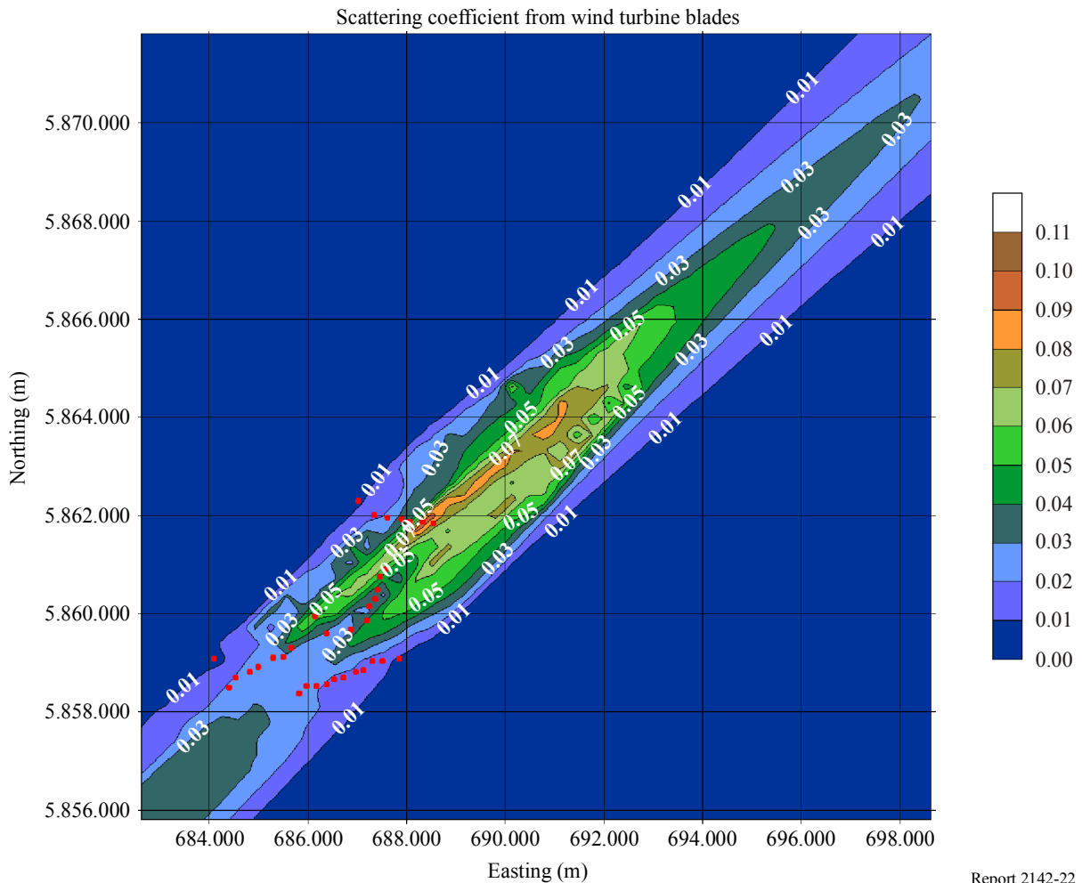
Calculated scattering coefficient from the blades of 35 wind turbines (red dots)
