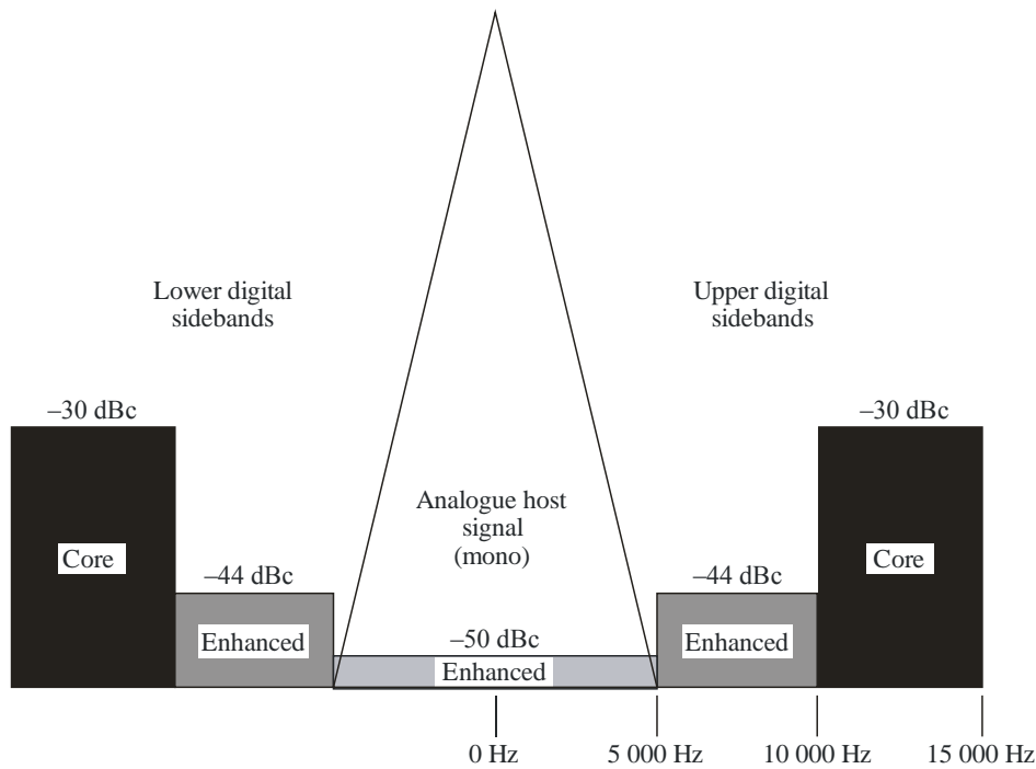
FIGURE 7 Hybrid MF IBOC DSB power spectral density
