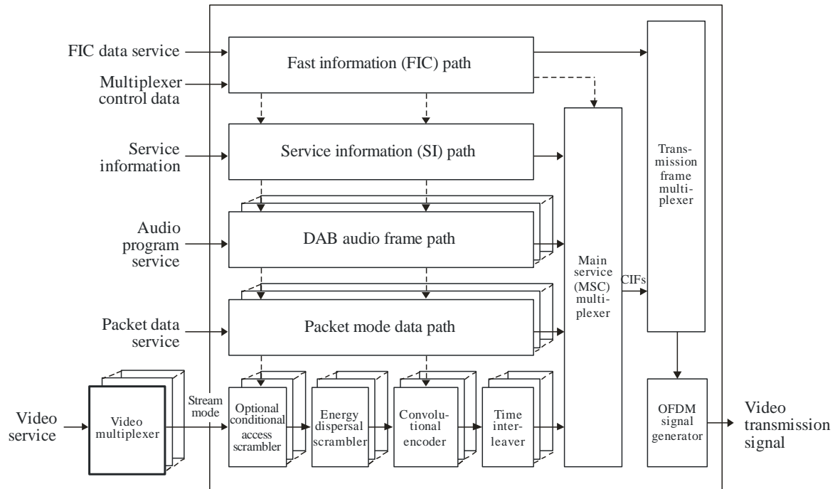
FIGURE 27 Conceptual transmission architecture for the video services DAB (ETSI EN 300 401)
