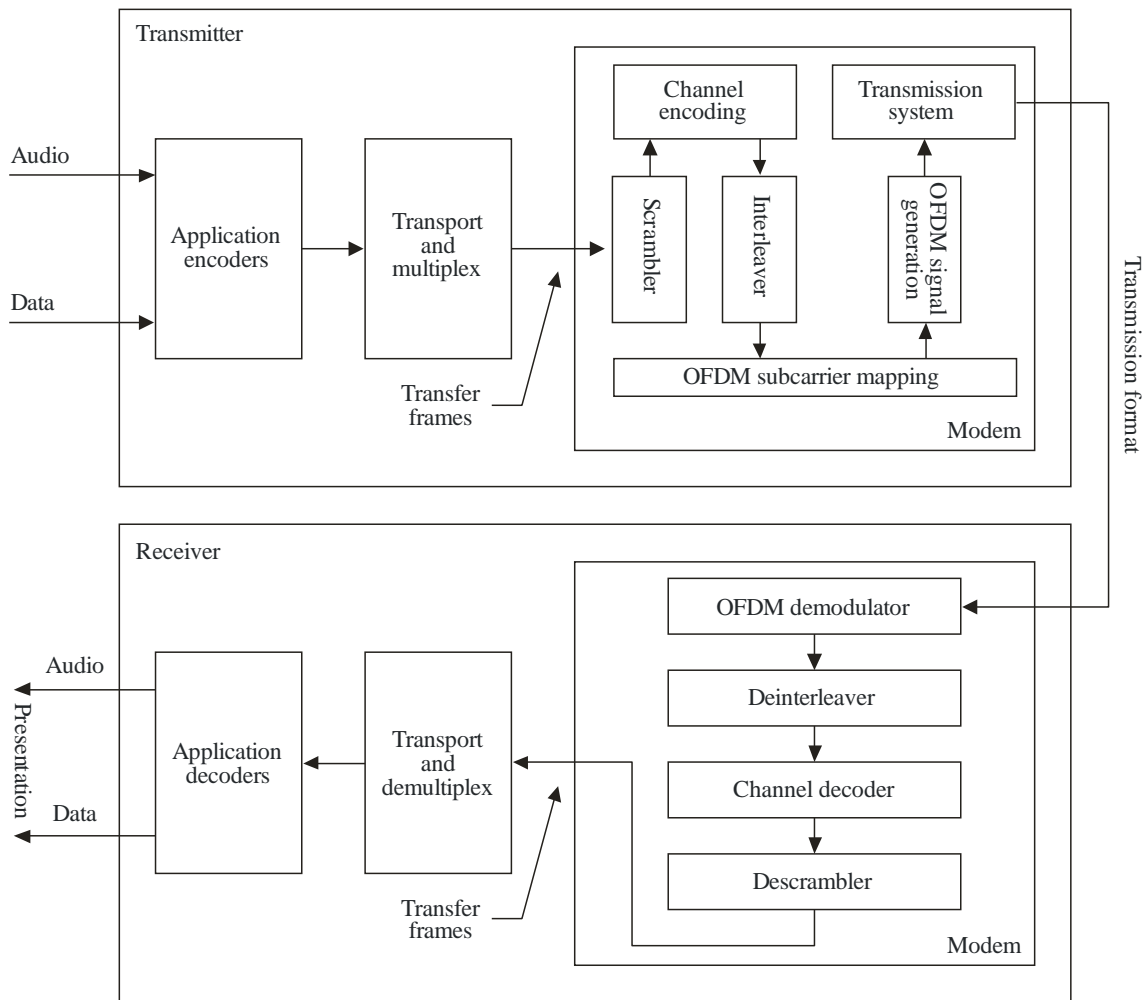
RF/Transmission function in context of overall system
