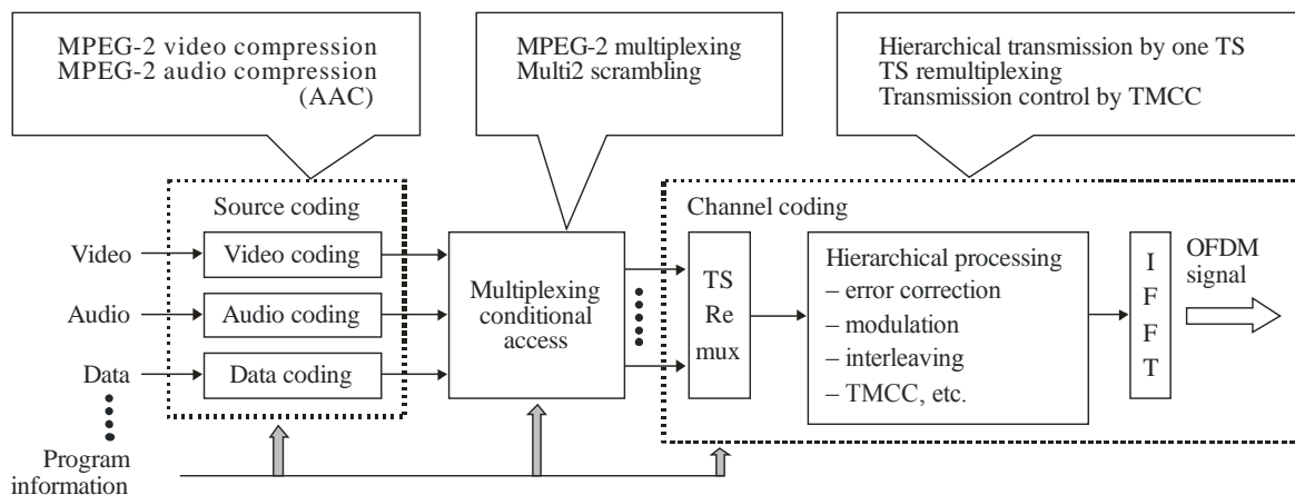
ISDB-T system configuration
