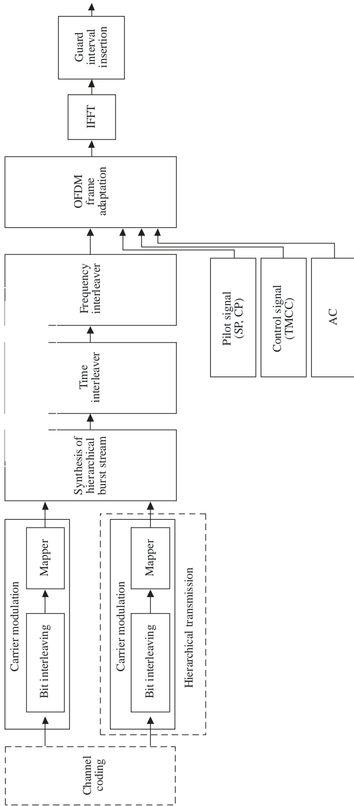
FIGURE 17 Modulation block diagram
