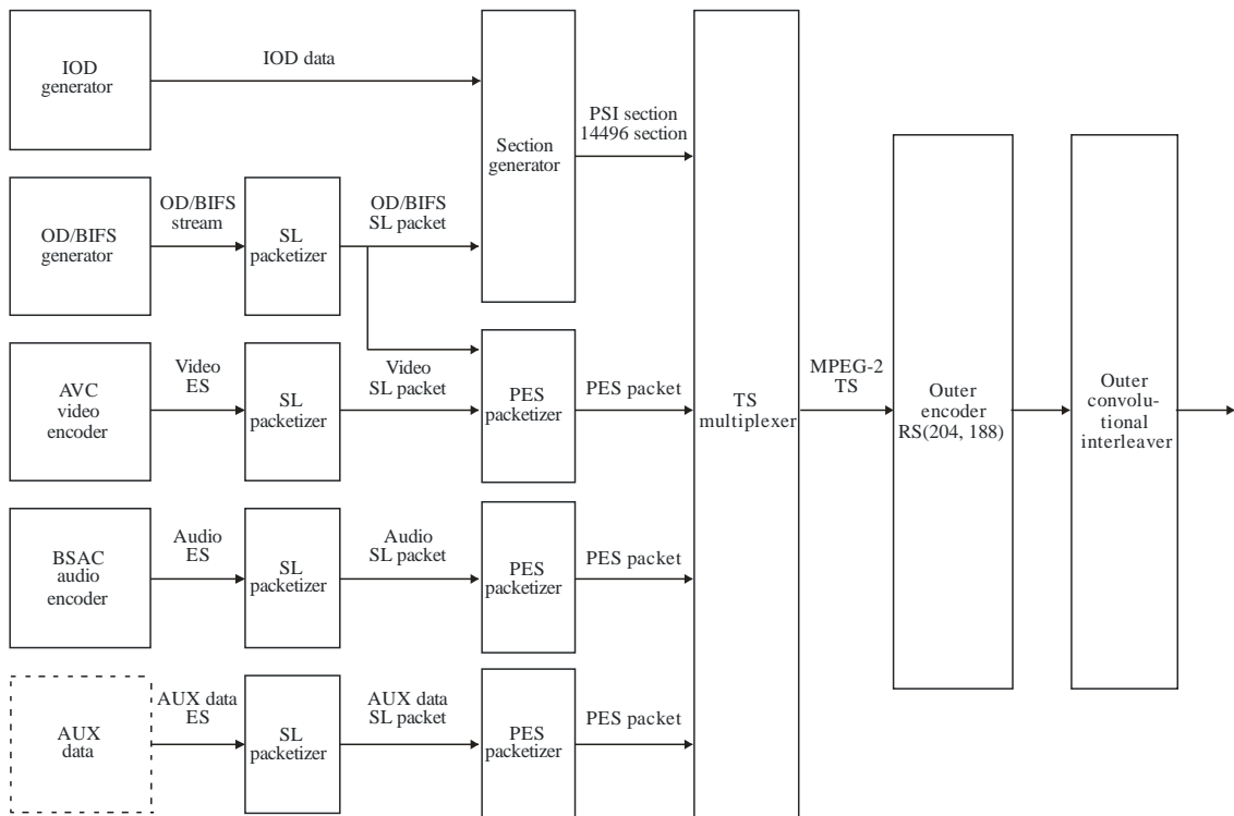
FIGURE 28 Architecture of the video multiplexer
