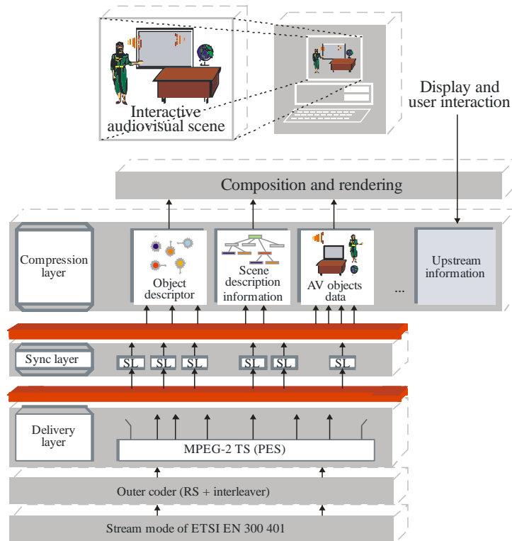
FIGURE 26 Conceptual architecture for the video services
