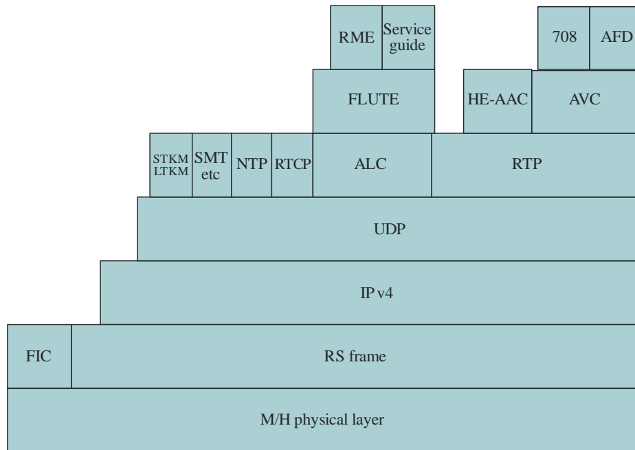
FIGURE 21 ATSC-M/H broadcast protocol stack
