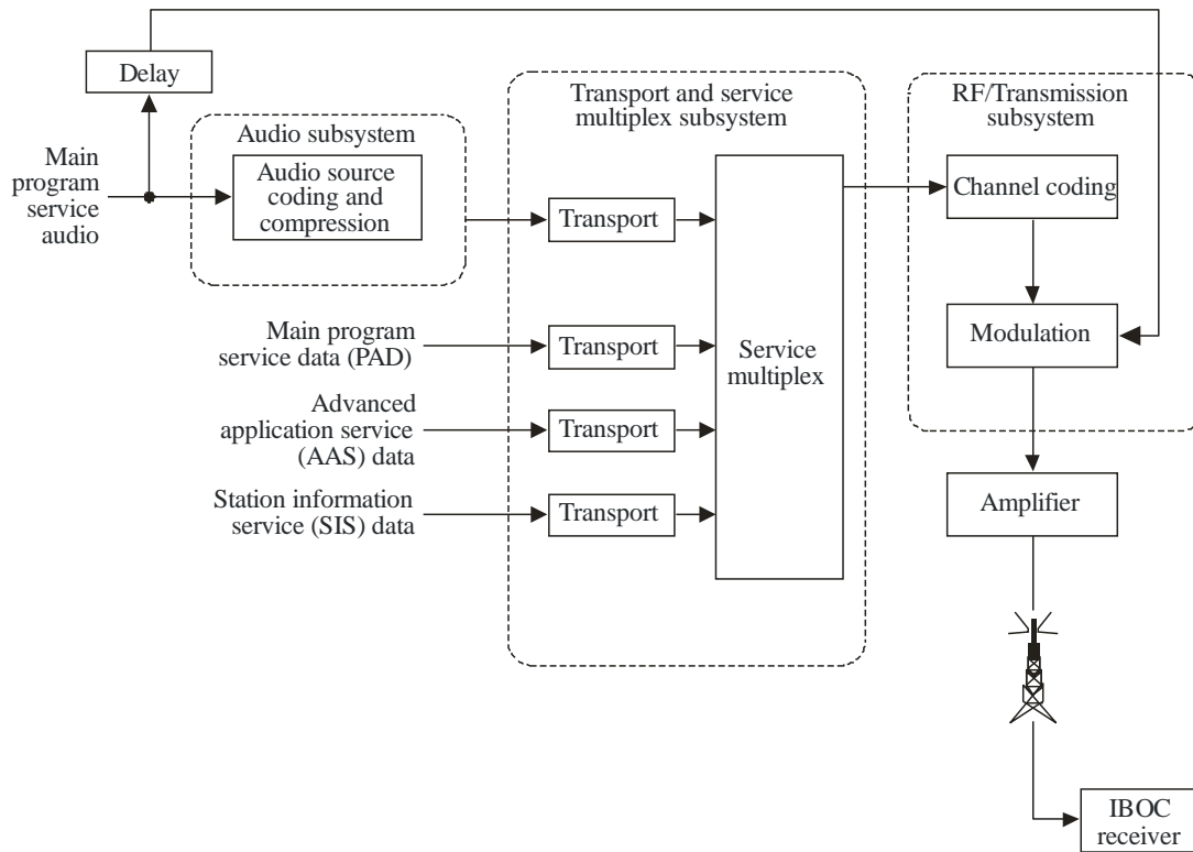
FIGURE 11 IBOC digital radio broadcasting model Analog audio (hybrid modes only)
