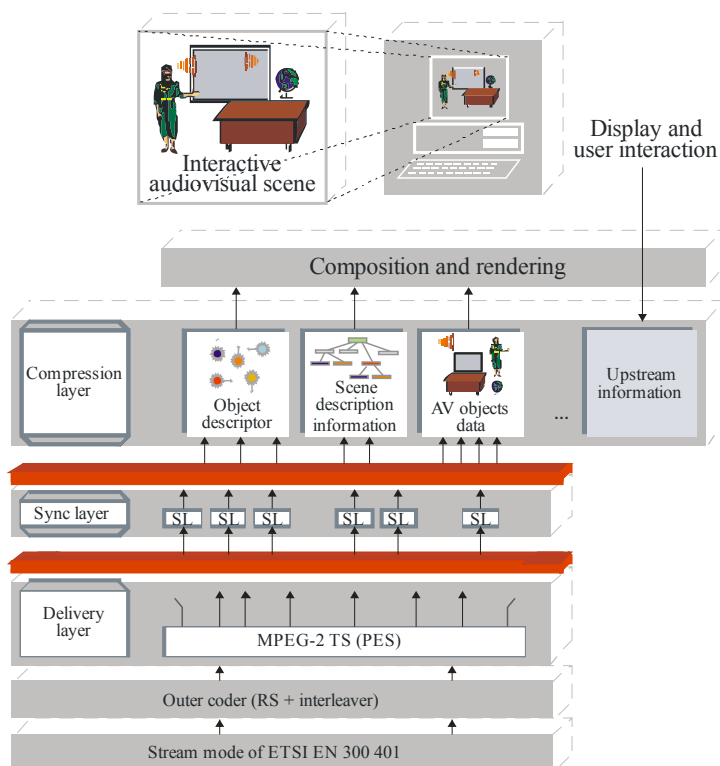
FIGURE 26 Conceptual architecture for the video services
