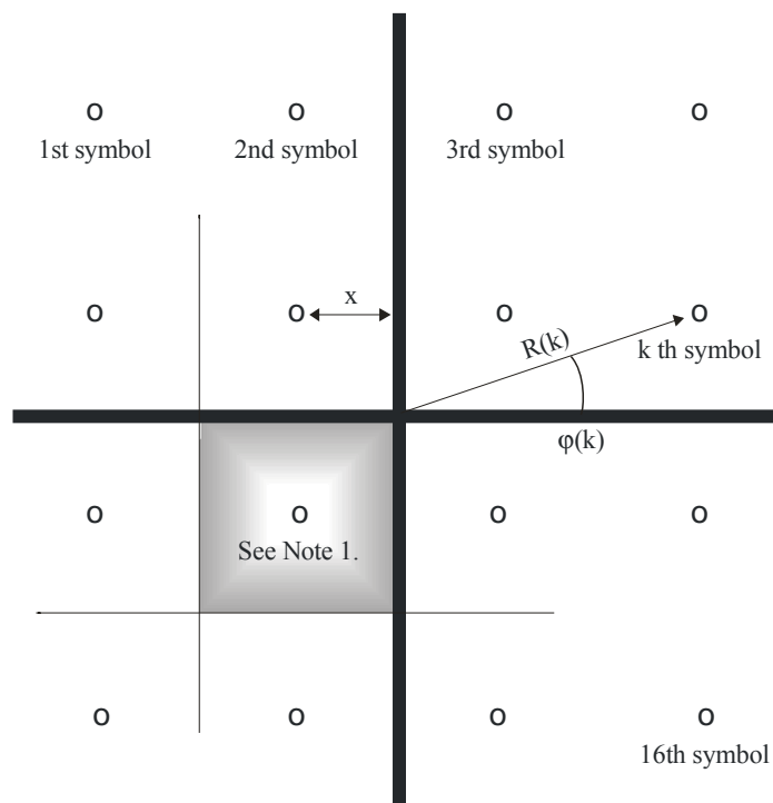
FIGURE 3 Constellation 16-QAM
