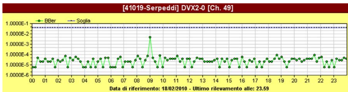
FIGURE 47 BER chart
