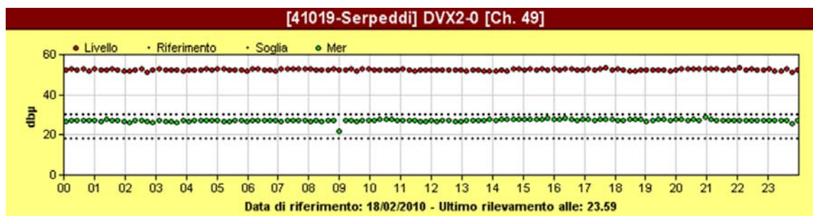
FIGURE 46 MER chart (threshold values are defined by ETSI)
