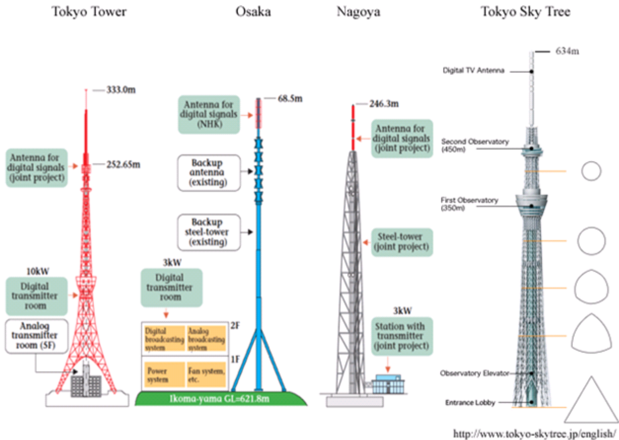
FIGURE 55 Digital transmitting facilities in major cities
