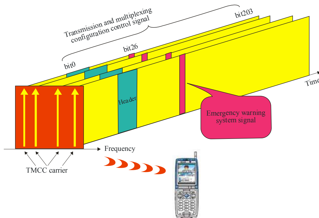
FIGURE 56 Activation of handheld receiver using EWS signals for digital terrestrial broadcasting
