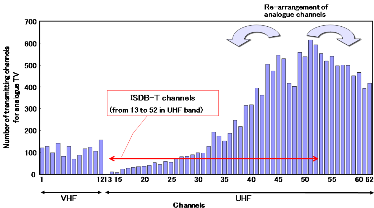
FIGURE 54 Number of transmitting channels for analogue TV
