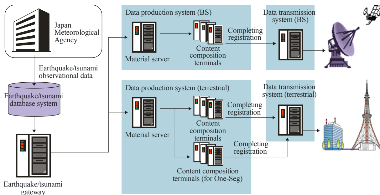
System configuration for earthquake and tsunami information
