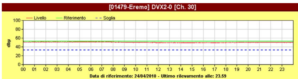
FIGURE 45 RF Charts
