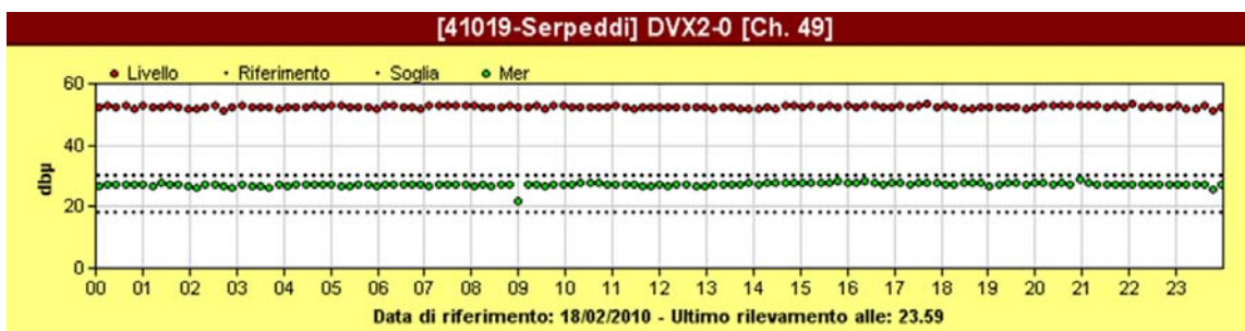
FIGURE 46 MER chart (threshold values are defined by ETSI)
