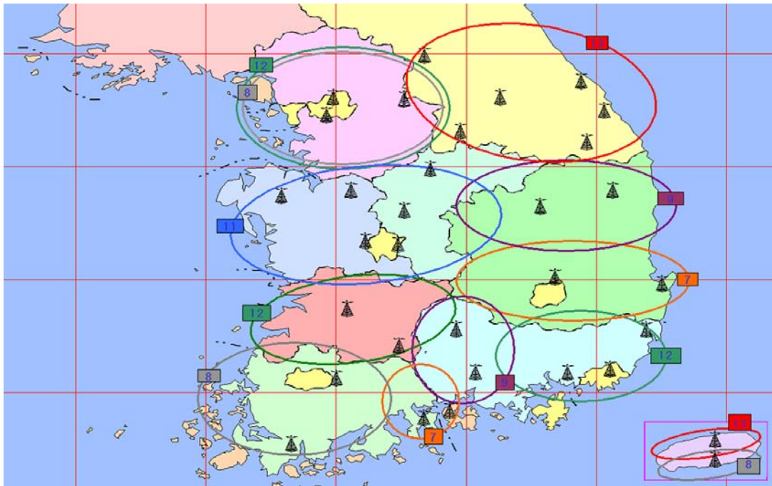
FIGURE 68 Channel Assignments for T-DMB in Korea
