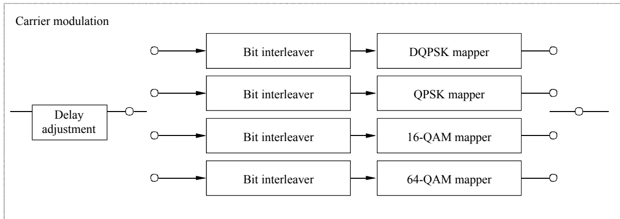
FIGURE 14 Configuration of carrier modulation block
