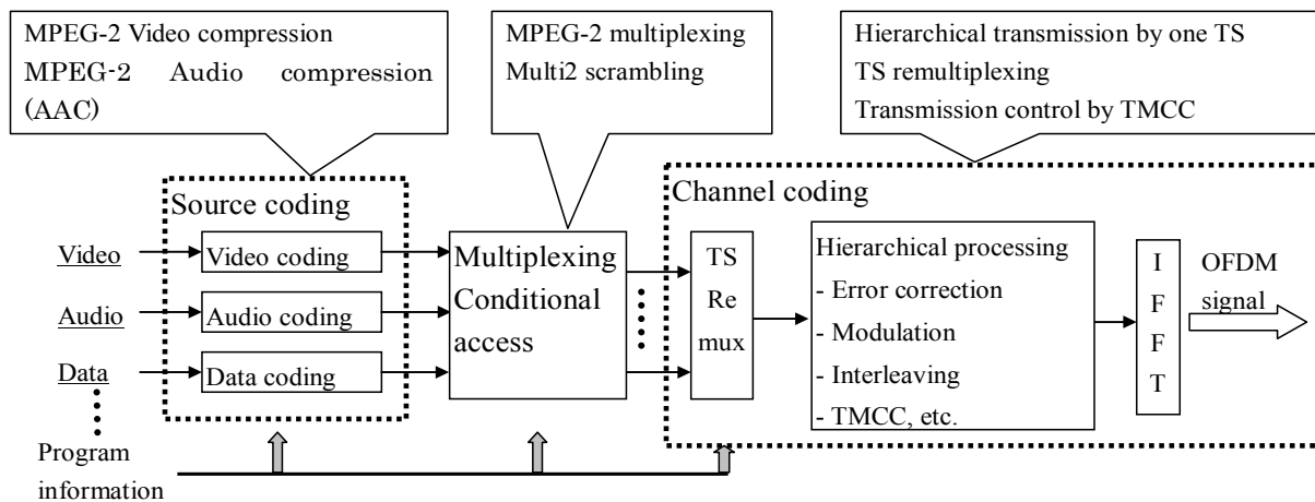
FIGURE 21 ISDB-T system configuration
