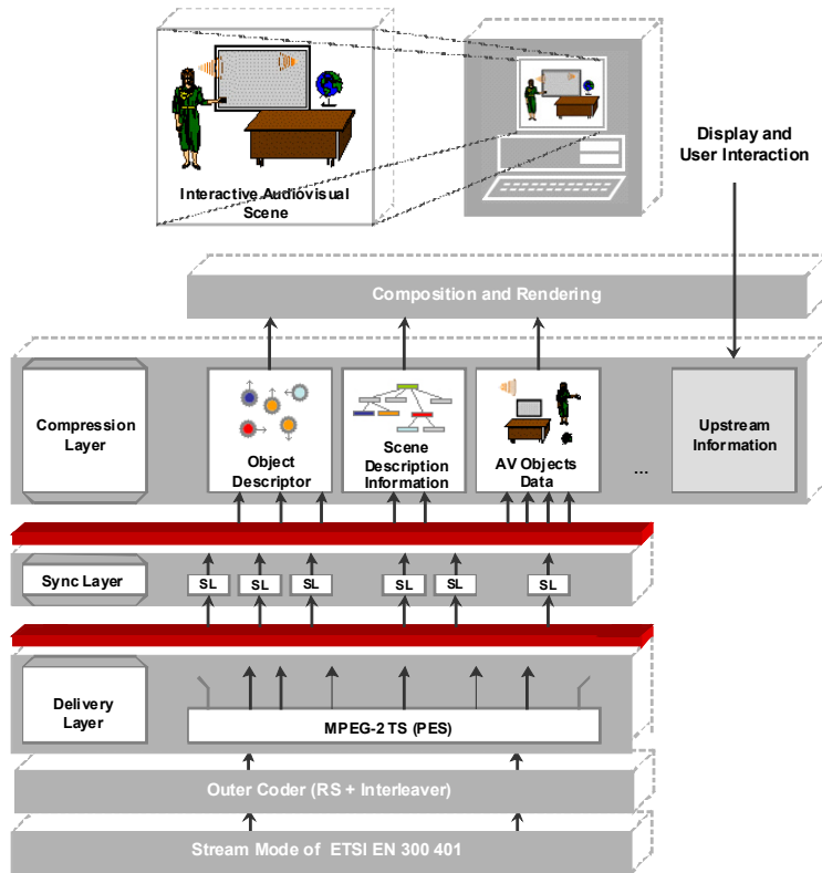
Conceptual architecture for the video services
