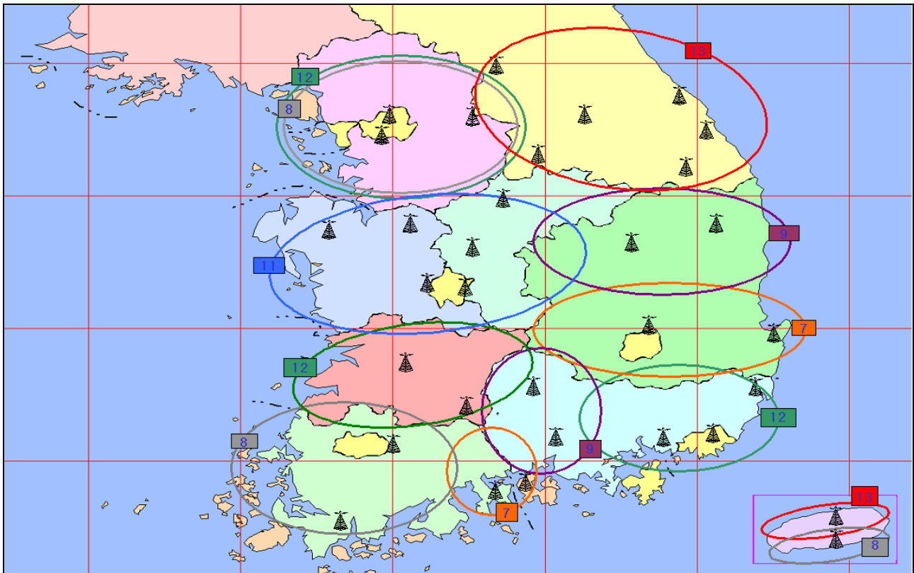
Channel Assignments for T-DMB in Korea
