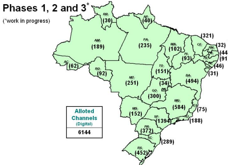
FIGURE 34 Digital channels allotted after the conclusion of Phase 3
