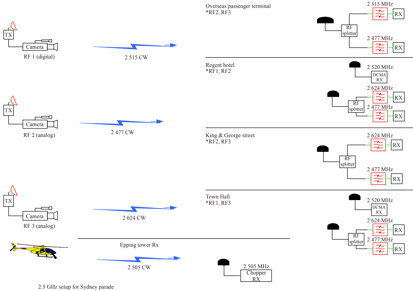
FIGURE 10 An Australian example of ENG/OB spectrum usage
