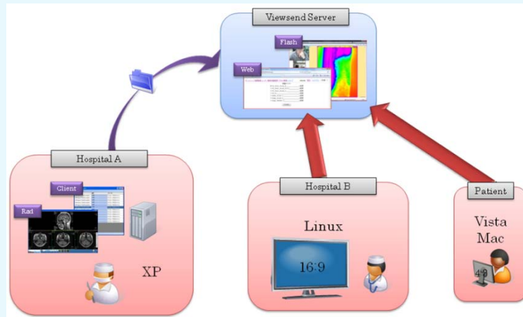
Figure 31: ViewSend Online
