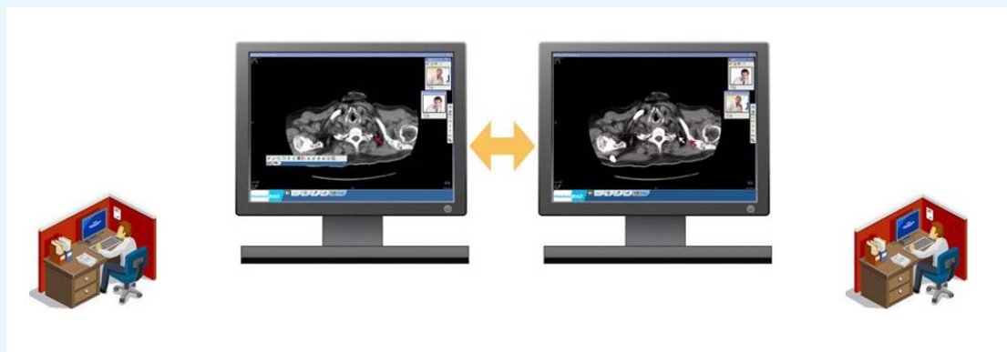
Figure 30: ViewSend videoconferencing
