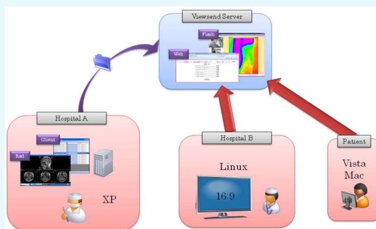
Figure 31: ViewSend Online
